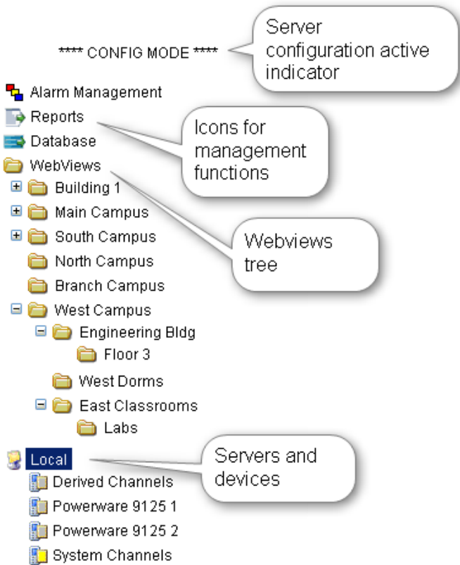
Figure 2 - Tree
