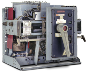
Original Magnetic Circuit Breaker
