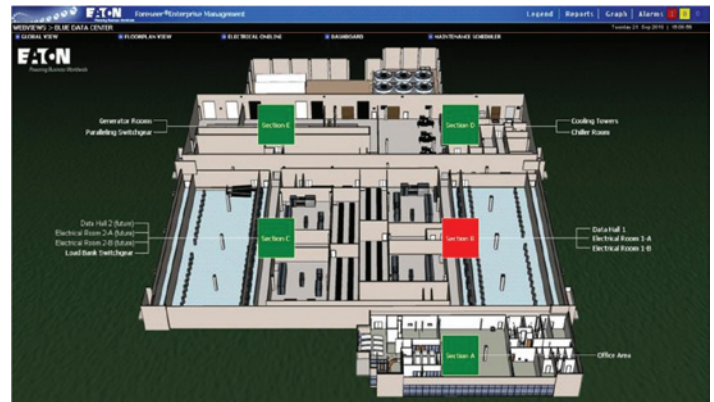
Foreseer is highly configurable to reflect the actual facility layout with alert tags.
