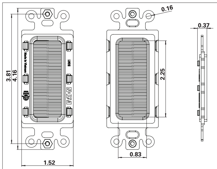
Figure 1. BIM1W dimensions
