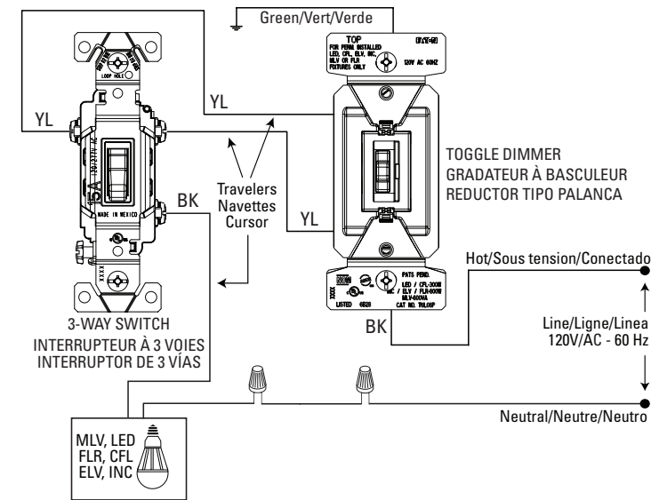
FIGURE 2: 3-WAY WIRING DIAGRAM FIGURE 2: SCHEMA DE CABLAGE DE 3-VOIES FIGURA 2: DIAGRAMA DE CABLEADO DE 3-VIAS
