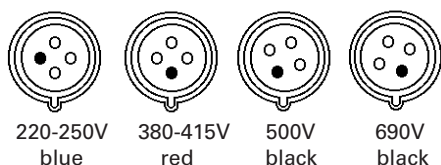
GHG 514, 4-pole 50/60Hz
