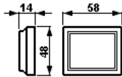
Front element of M45 measuring instrument
