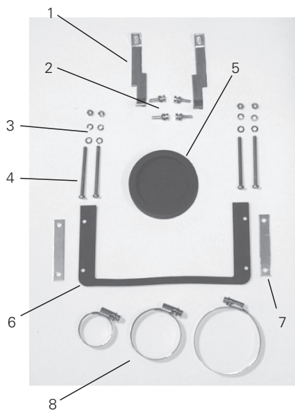
Assembly pieces of the double cable end box
