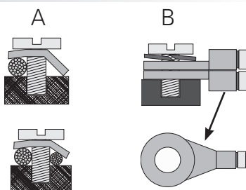
Fig. 1.3.a Connection Main-; Aux.-/Signal contact
