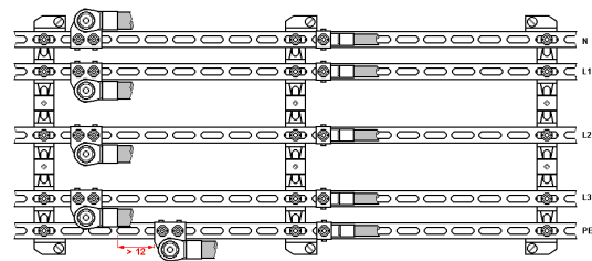
Fig. 3 Bus bar system – vertical connection
