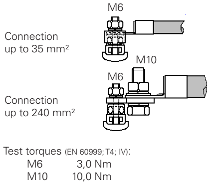
Fig. 1 Connection diagrams
