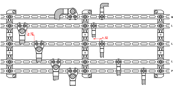
Fig. 1.3.a Connection Main-; Aux.-/Signal contact
