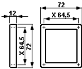
Front element of M72 measuring instrument
