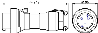
Plug 3-pole
