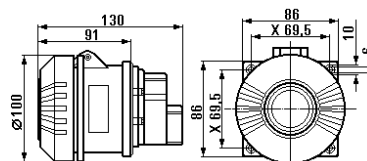
Flange socket 5-pole
