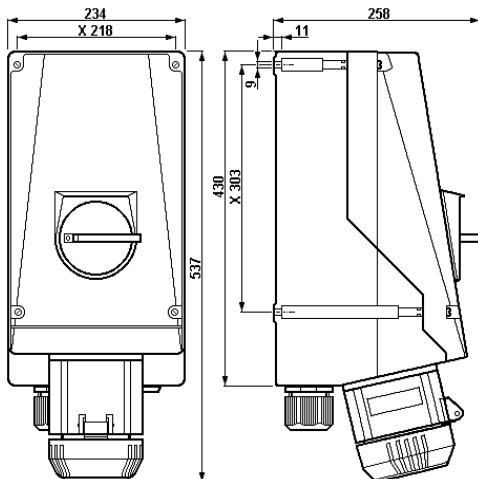
Wall socket
