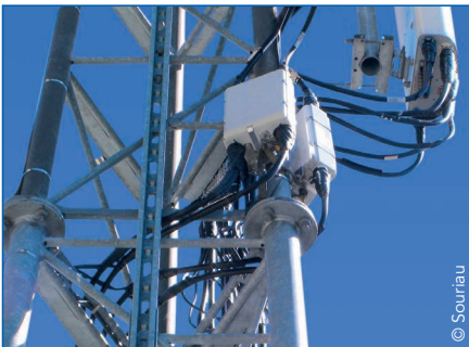
Cell Tower Distribution Box
