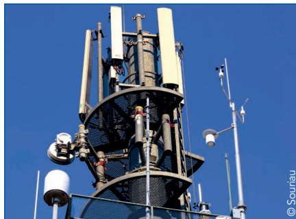
Remote Radio Head
