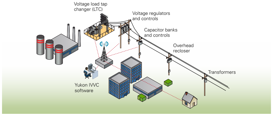
Typical diagram illustrating how Yukon IVVC application works within a power distribution system
