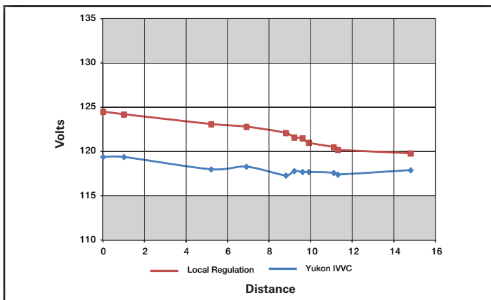
Voltage Profile: Local Regulation vs Yukon IVVC
