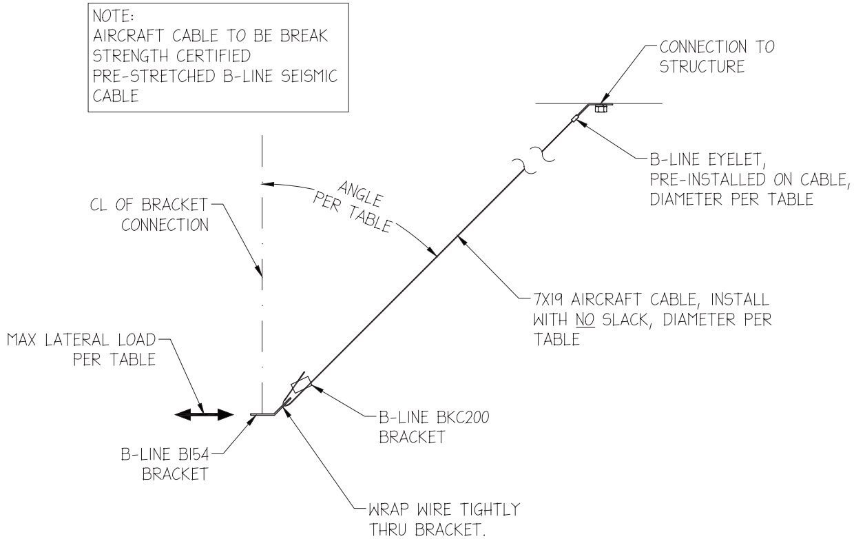
CABLE BRACE B154 BRACKET AND EYELET ASSEMBLY SCALE: 1/2"=1'-0"
