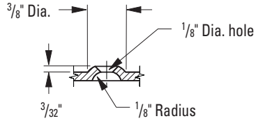
Button detail
