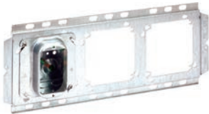
BB816-204DA-1-X-X
