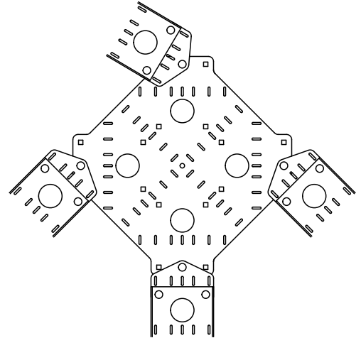
OPTIONAL PIVOT CONNECTOR ATTACHMENT (6" WIDTH SHOWN)
