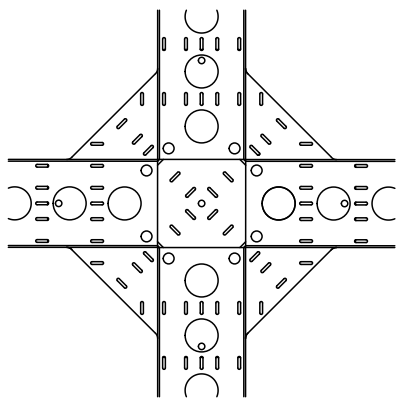
0" RADIUS ATTACHMENT (6" WIDTH SHOWN)
