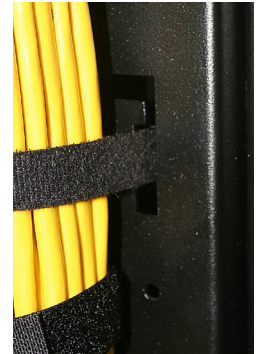
Velcro Straps can be used to secure cables using the cut-out pattern.
