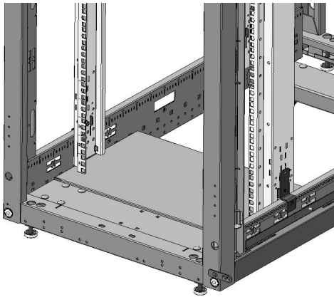
Bottom horizontal panel (600 mm) Kit # RSHP6XX
