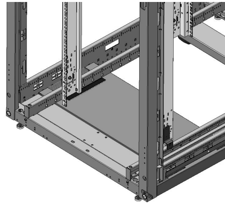
Bottom horizontal panel (800 mm) Kit # RSBPAIRD2
