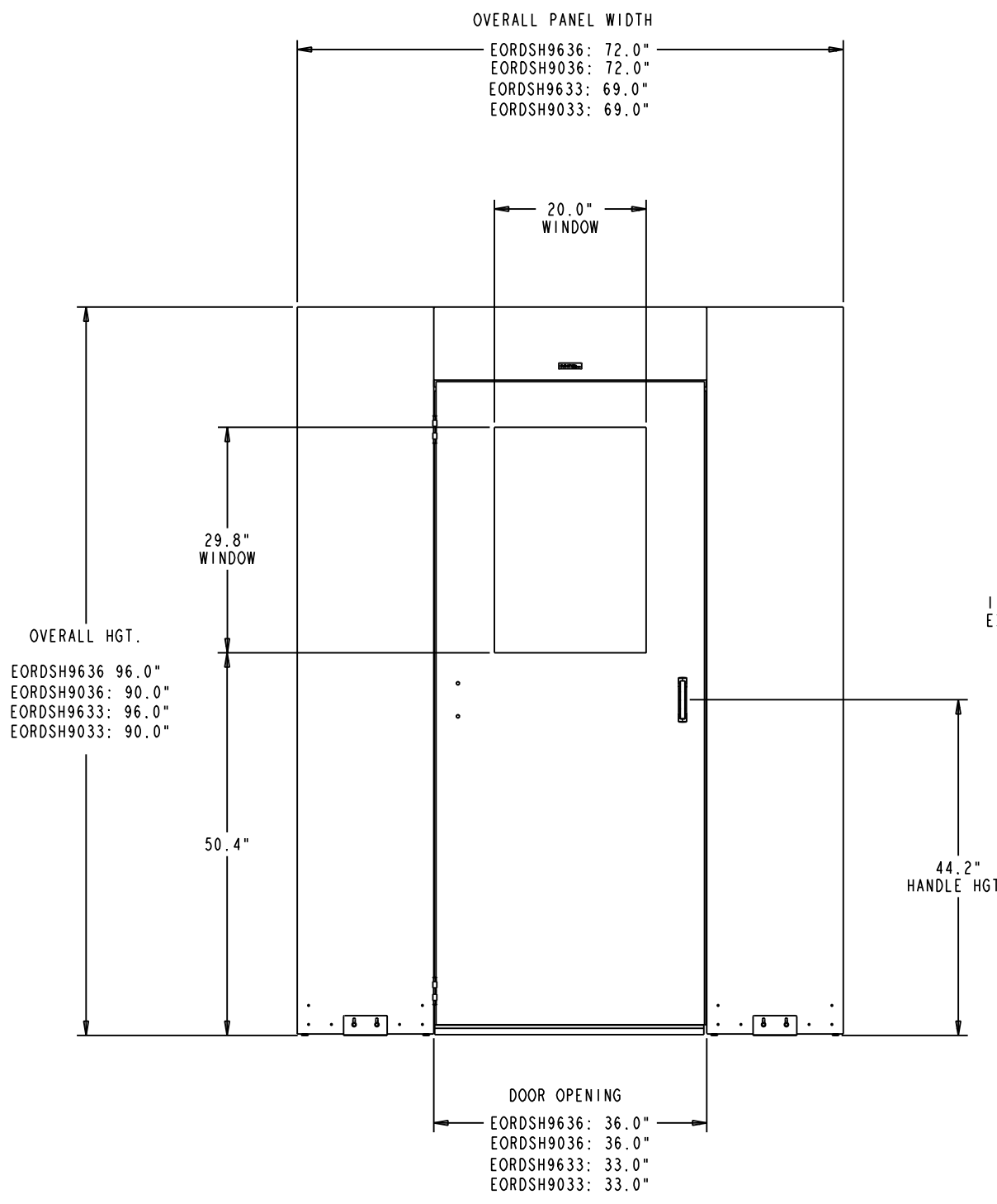
DOOR CLOSED
