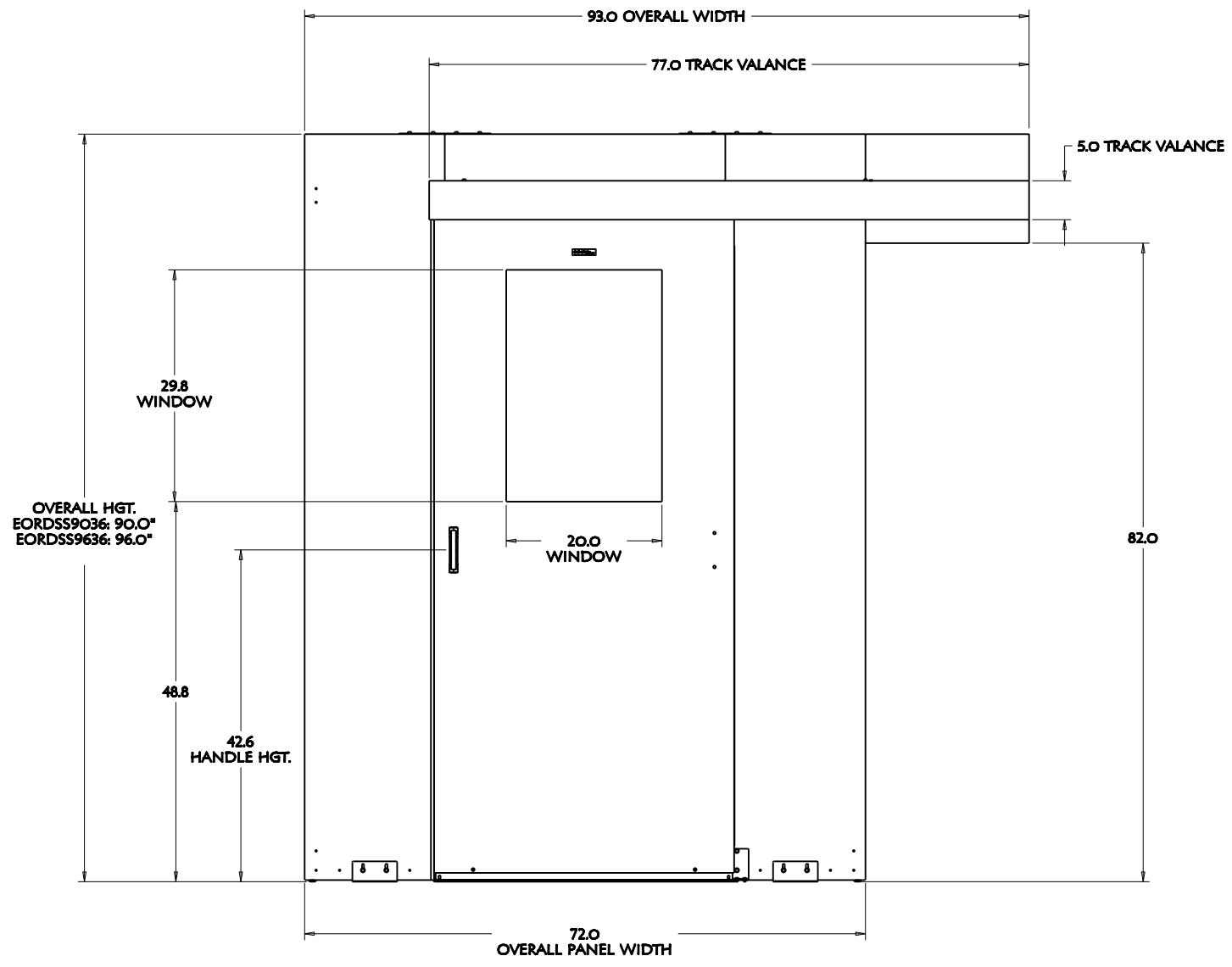
DOOR CLOSED
