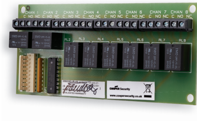
8600 relay card
