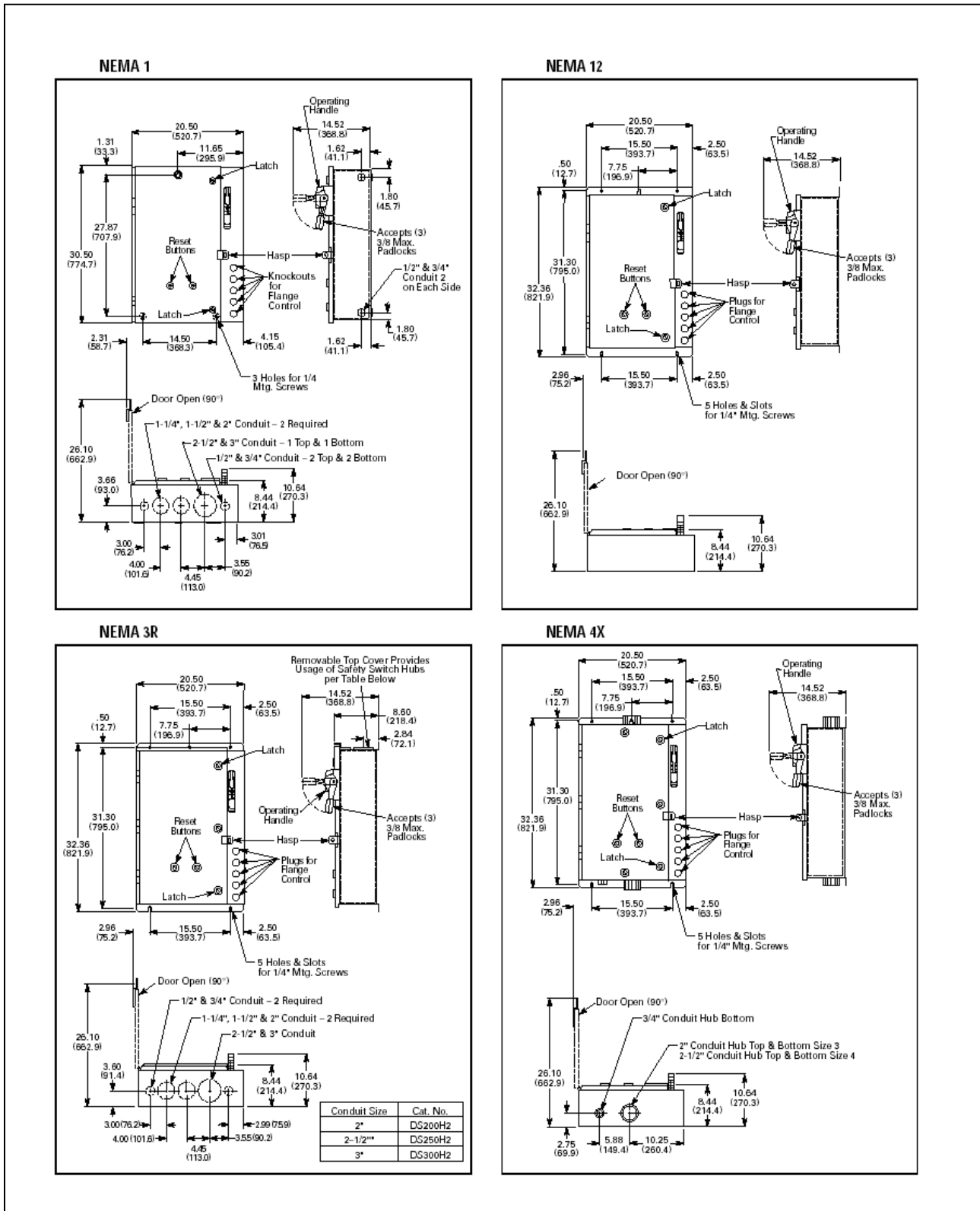
FIGURE 1: TYPICAL DIMENSION DRAWING
