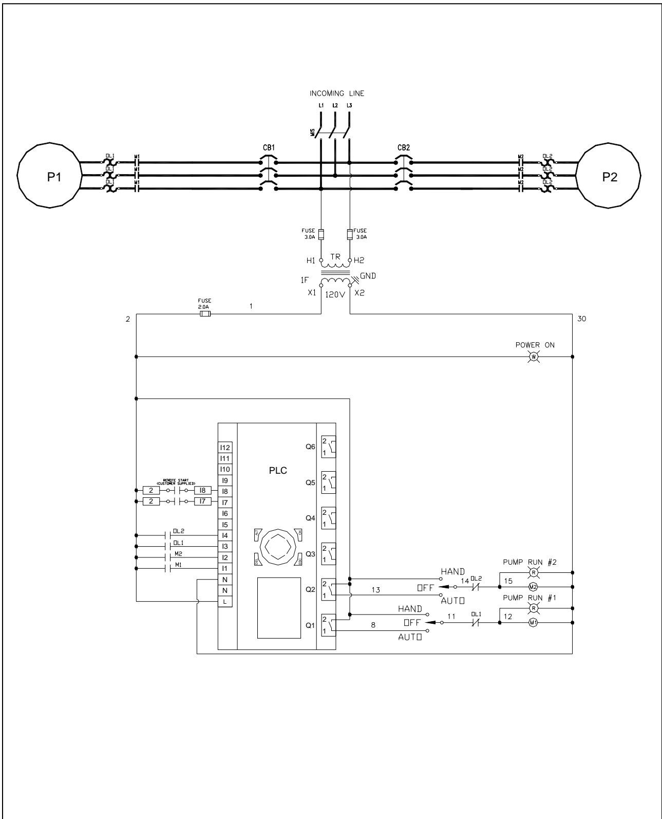
FIGURE 2: TYPICAL WIRING SCHEMATIC – PLC Based Controller
