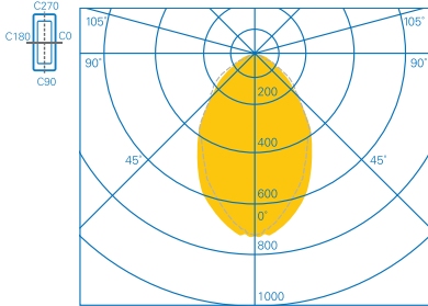
Ceiling mounting, Open area, HiBay
