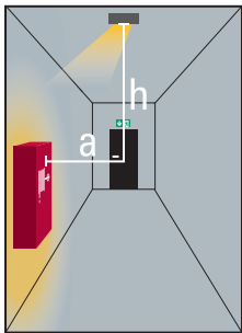
200lm with maintenance factor 0.94
