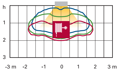
200lm with maintenance factor 0.94
