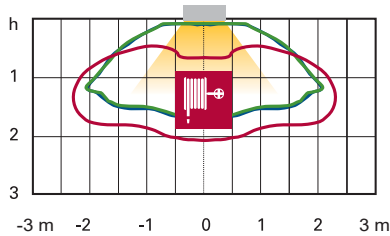
400lm with maintenance factor 0.94
