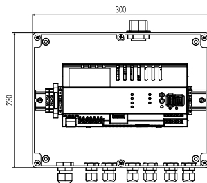
Dimensional drawings, data in mm
