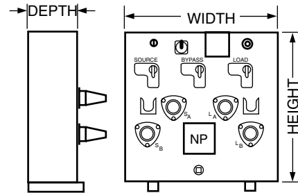
Figure 3. Bypass switch module (optional).
