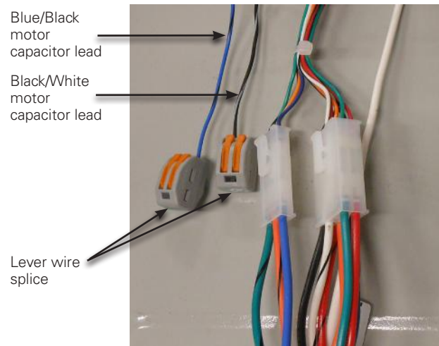
Figure 41. Capping the motor capacitor wires.
