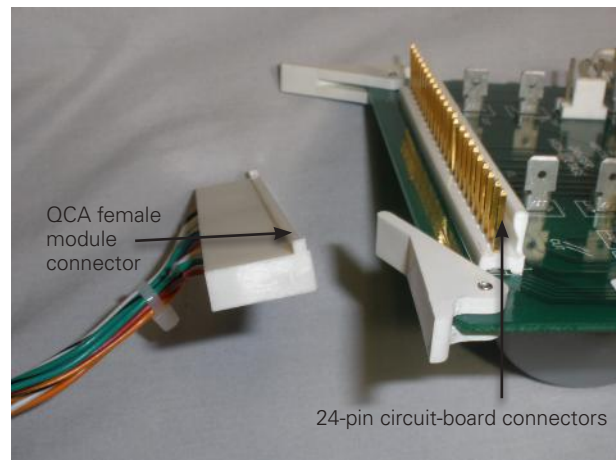
Figure 35. Alignment of QCA and circuit-board connectors.
