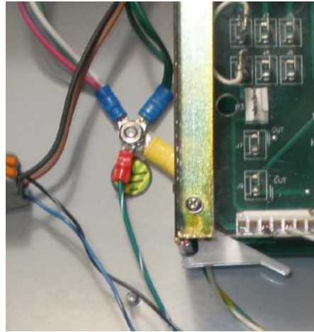
Figure 47. Connecting the shielding wire, General Electric.
