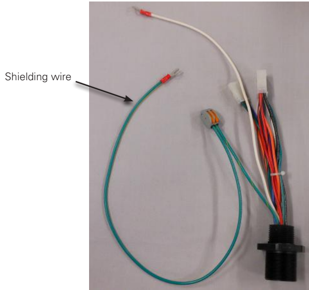
Figure 46. Pigtail harness with green/yellow shielding wire.
