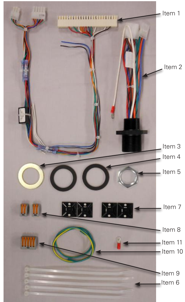
Figure 27. GE pin terminal QCA kit.
