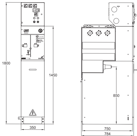
Type K panel dimension for 12kV
