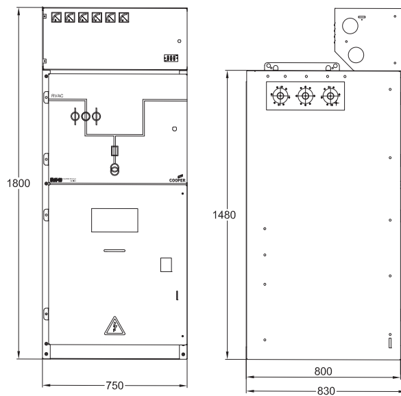
Type M panel dimension for 12kV
