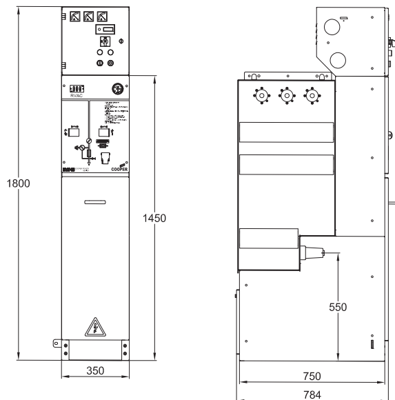
Type T panel dimension for 12kV
