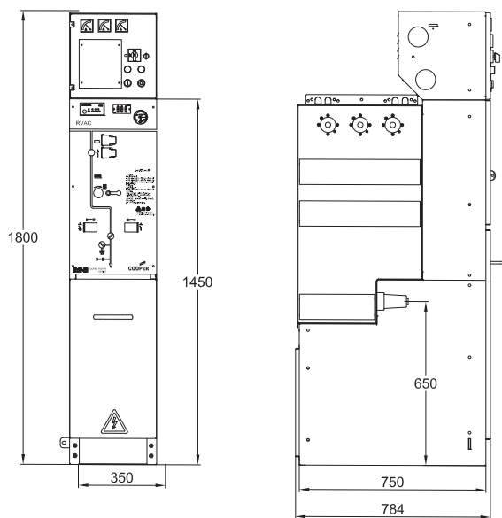
Type V panel dimension for 12kV
