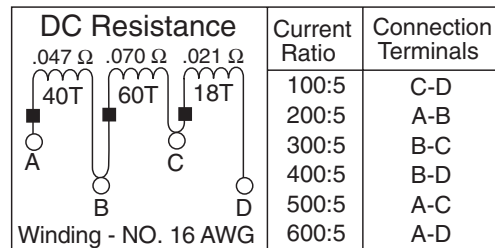
Figure 6. Current ratios and connection terminals for KA712L2S, KA712L3S, and KA712L5S
