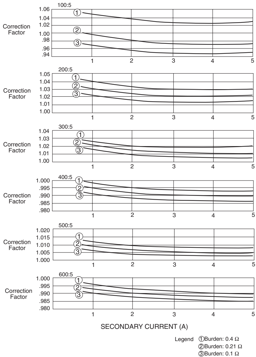
Figure 8. Correction curves for 600:5 multi-ratio bushing current transformer, Catalog Numbers KA712L2S, KA712L3S, and KA712L5S
