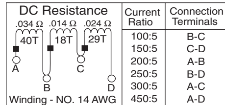
Figure 5. Current ratio and connection terminals for KA712L1S
