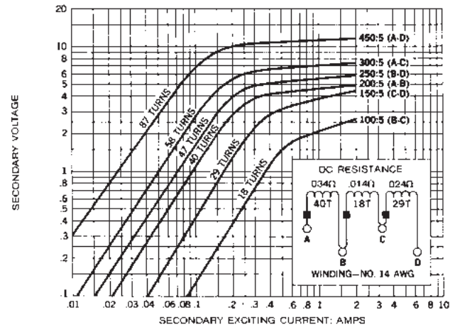
Figure 9. Typical secondary excitation curves for 450:5 Multi-ratio “Slip-on” Bushing Current Transformer, Catalog No. KA712L1S.
