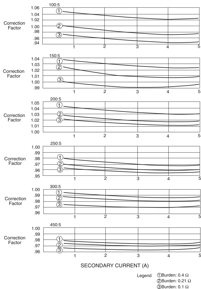
Figure 7. Correction curves for 450:5 multi-ratio bushing current transformer, Catalog No. KA712L1S
