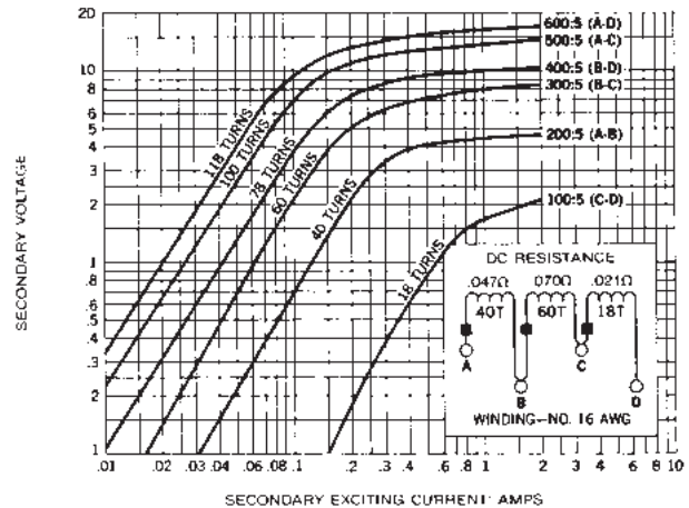
Figure 10. Typical secondary excitation curves for 600:5 Multi-ratio “Slip-on” Bushing Current Transformer, Catalog Numbers KA712L2S, KA712L3S, and KA712L5S
