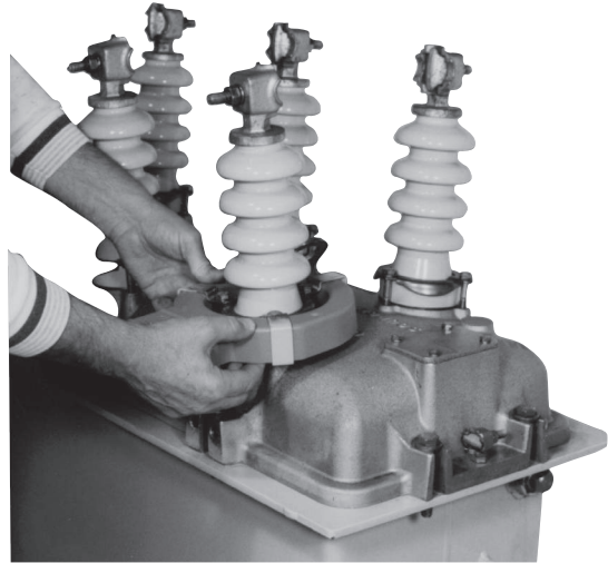
Figure 3. Mounting clamp is clipped to CT assembly and attached under bushing clamping bolt
