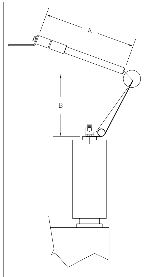
Figure 2. Expulsion Fuse Mounting Configuration - Vertical Orientation
