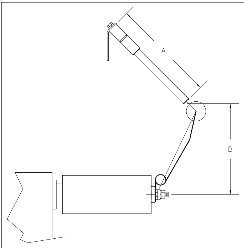
Figure 1. Expulsion Fuse Mounting Configuration - Horizontal Orientation
