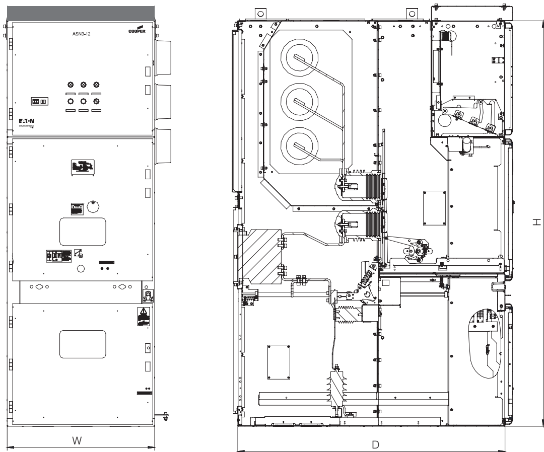
Drawing of ASN3 switchgear dimensions and structure
