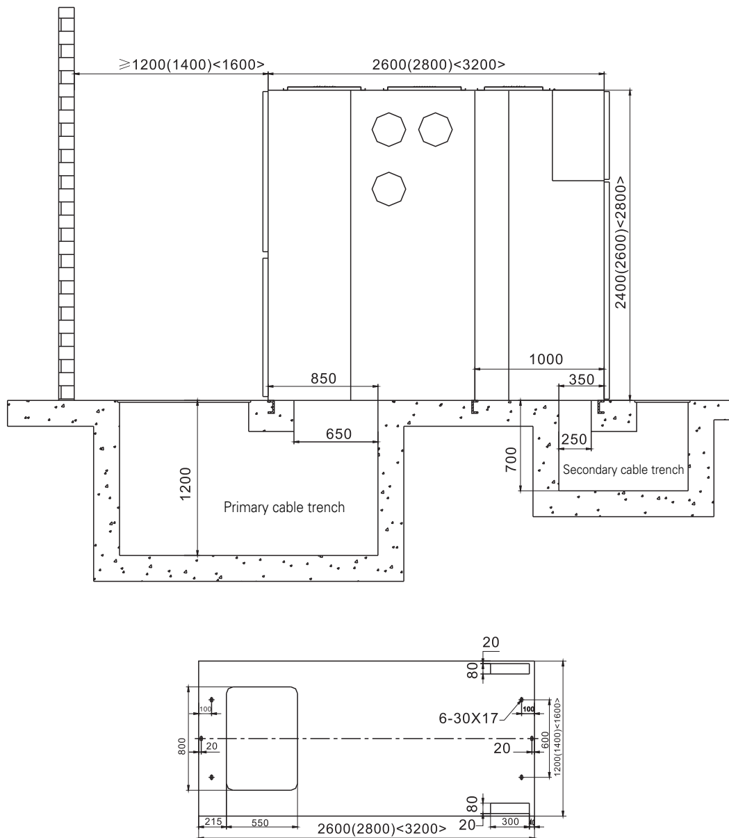
Drawing of installation foundation and sizes of holes of bottom plate for ASN1 switchgear
