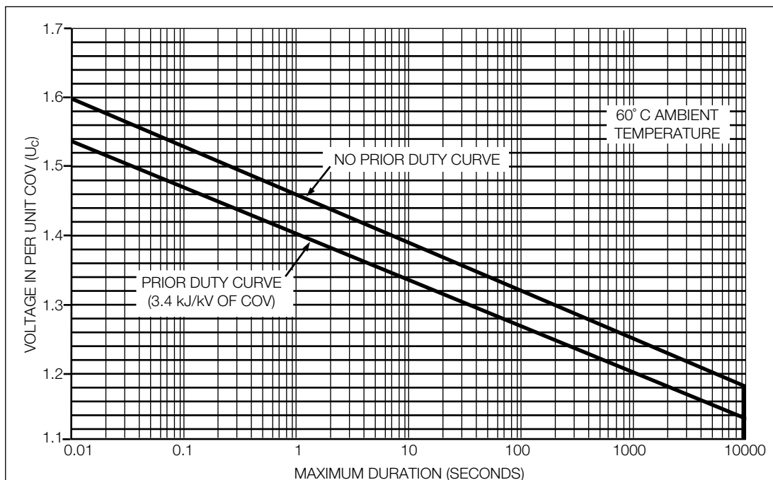
Figure 2. Temporary overvoltage capability of VariSTAR AZG2 surge arresters.
