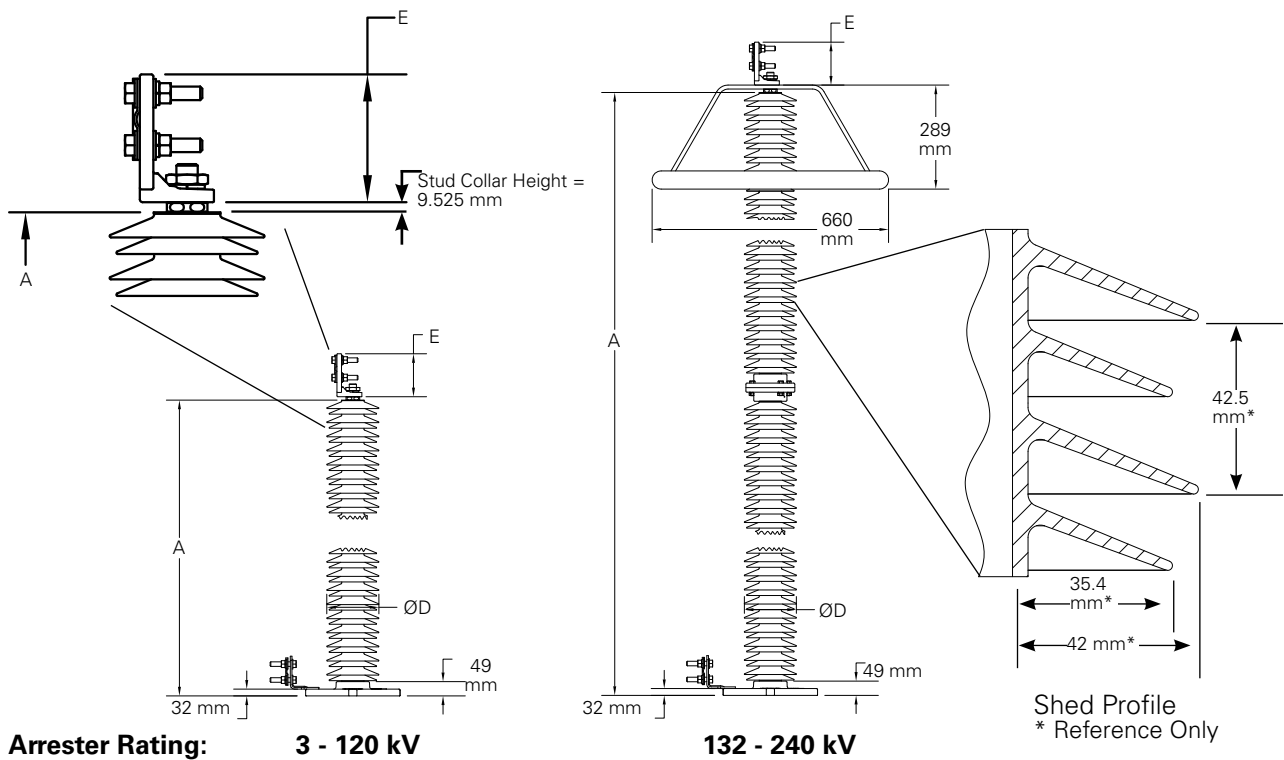
Figure 4. Outline Drawing of Standard UltraSIL Polymer-Housed VariSTAR Type U4 Surge Arresters.
