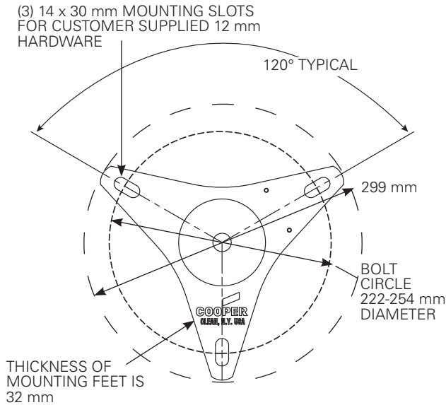
Figure 5. Base mounting.
