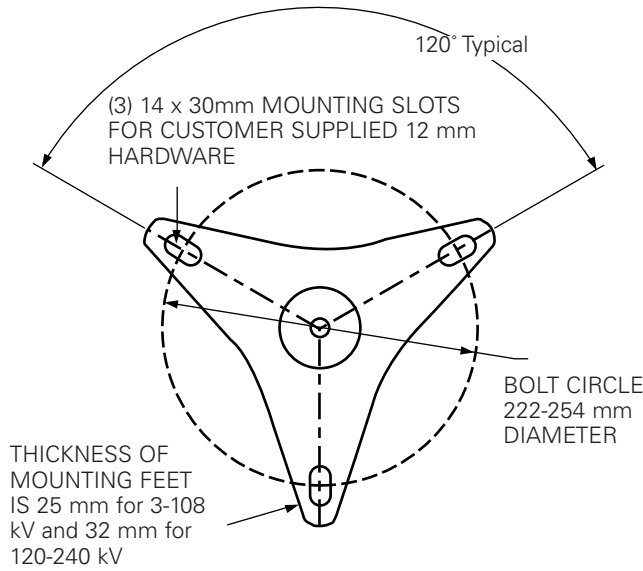
Figure 7. Base mounting.
