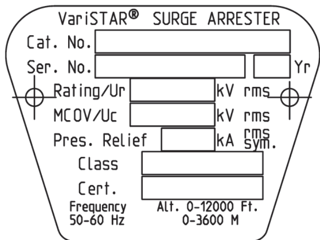
Figure 5. Arrester base nameplate (English version).
