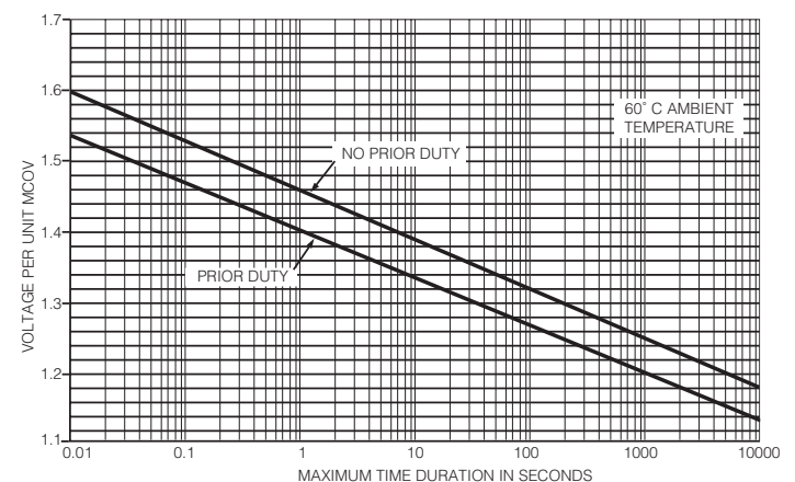
Figure 3. Temporary Overvoltage Capability of VariSTAR U2 Surge Arresters.
