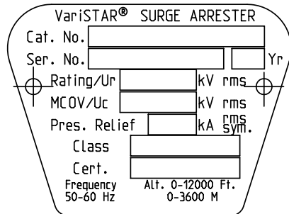
Figure 6. Detail of base nameplate.
