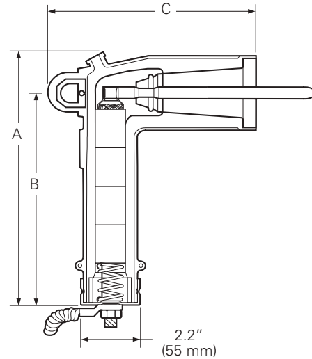
Figure 3. Dimensional information of POSI-BREAK M.O.V.E. surge arrester (refer to Table 4).
