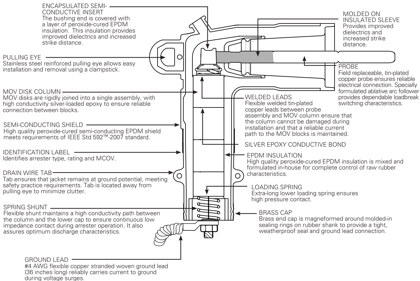
Figure 1. Cutaway illustration shows 25 kV Class POSI-BREAK M.O.V.E. surge arrester.
