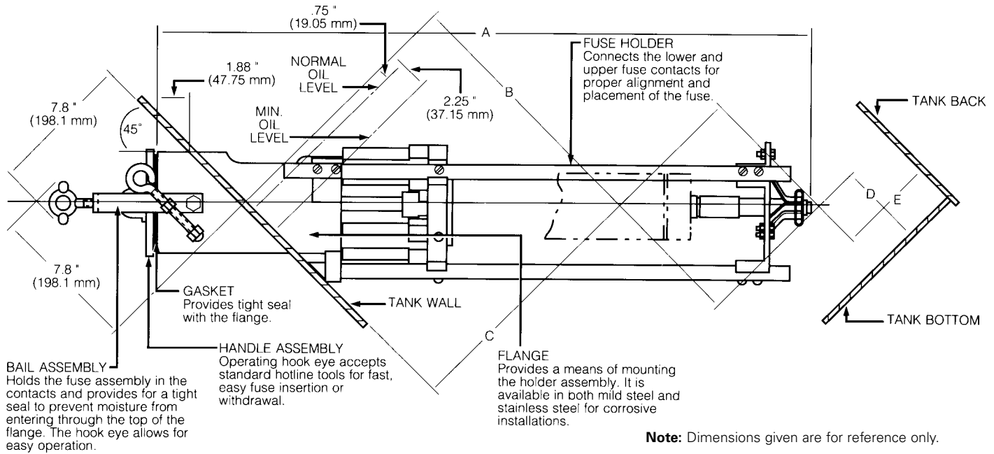
Figure 1. Dimensional information for ELSG Fuse Holder.
