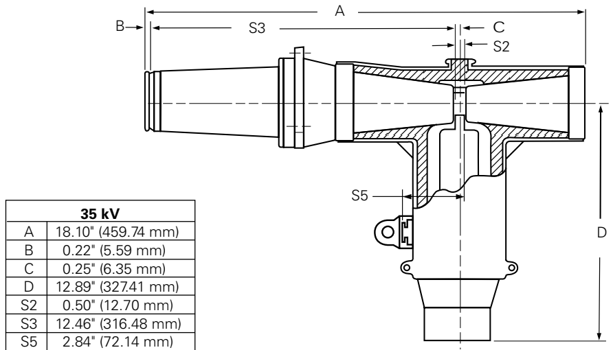
Figure 2. T-OP II connector profile and stacking dimensions.
