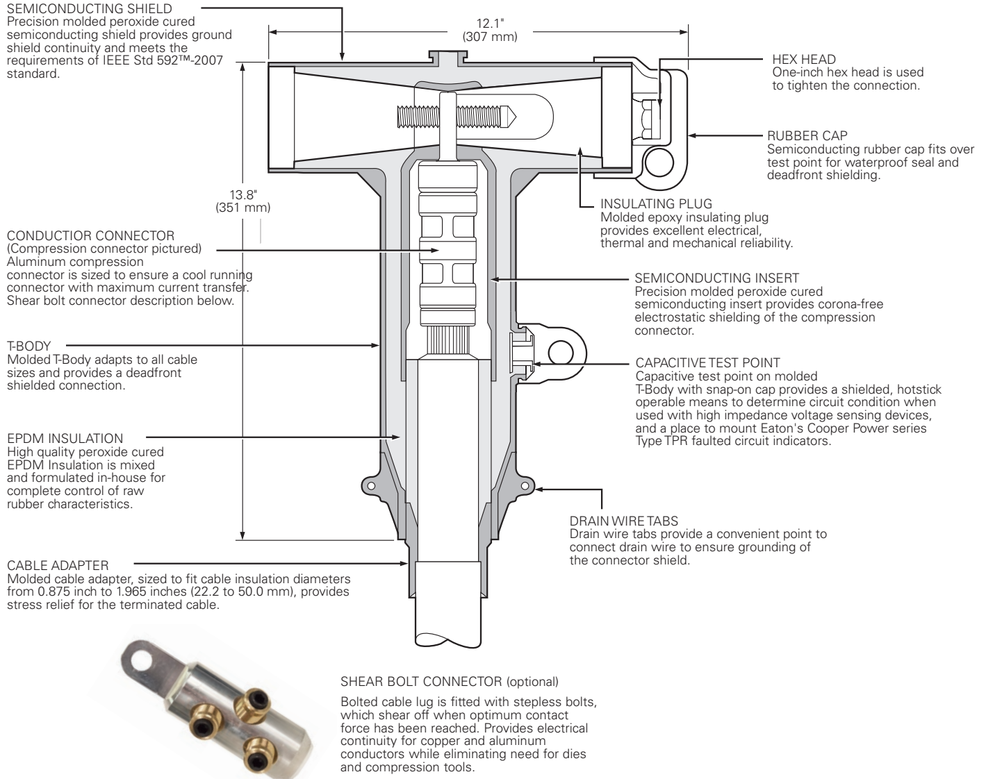
Figure 1. BOL-T cutaway illustrates design features.
