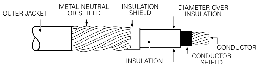
Figure 2. Illustration showing typical construction of medium voltage underground cable.
