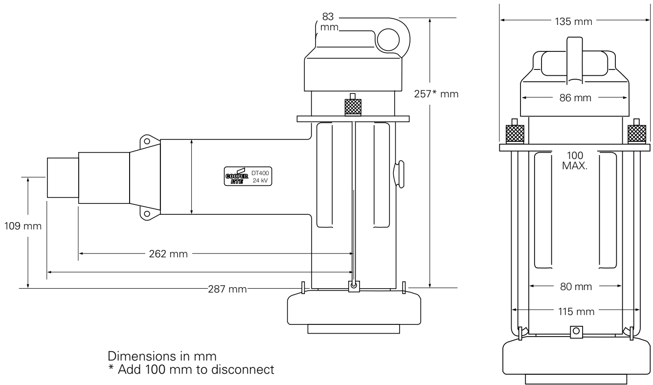
Figure 3. DT400P Deadbreak Tee Connector dimensional information.
