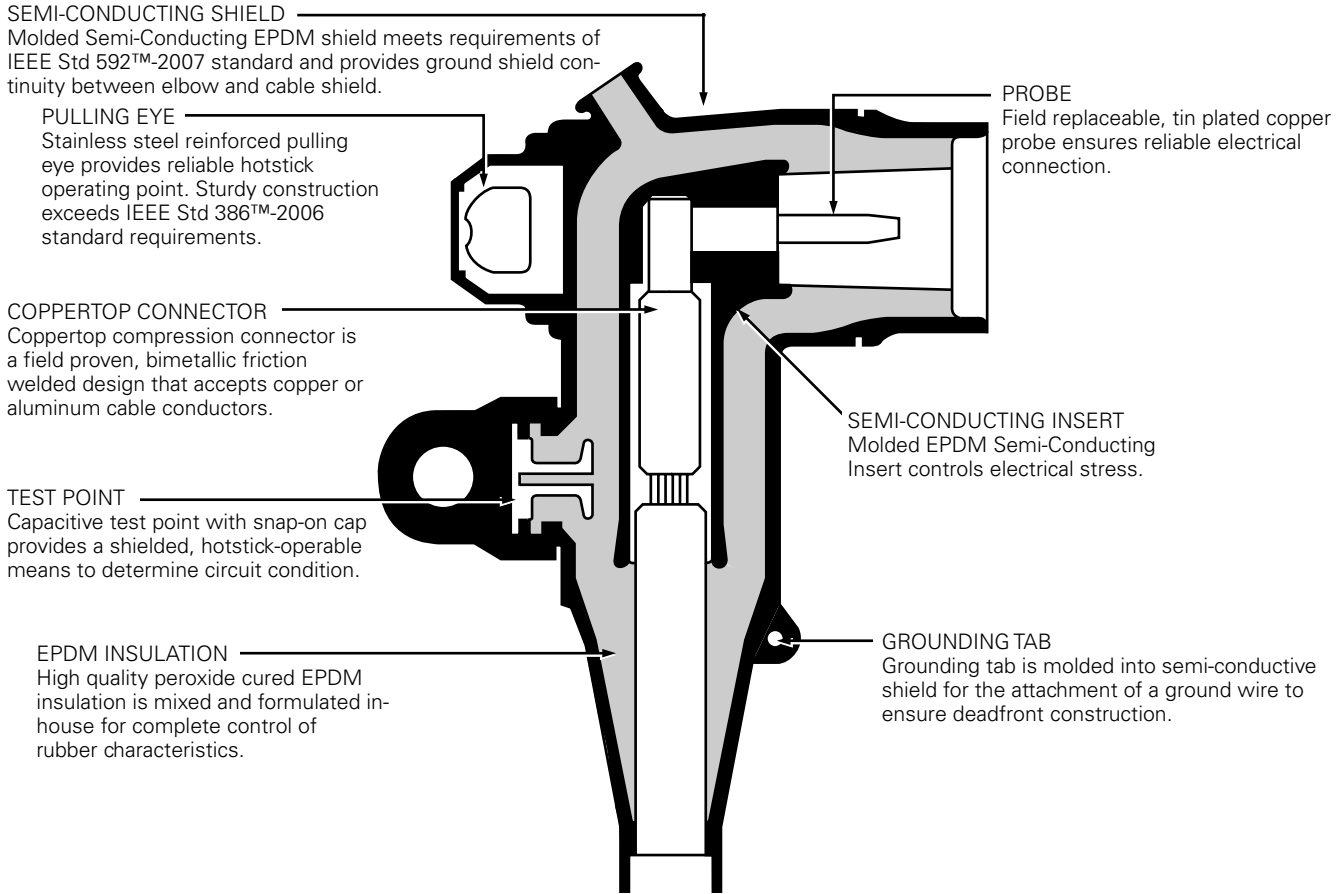
Figure 1. Elbow cutaway illustrates design integrity.
