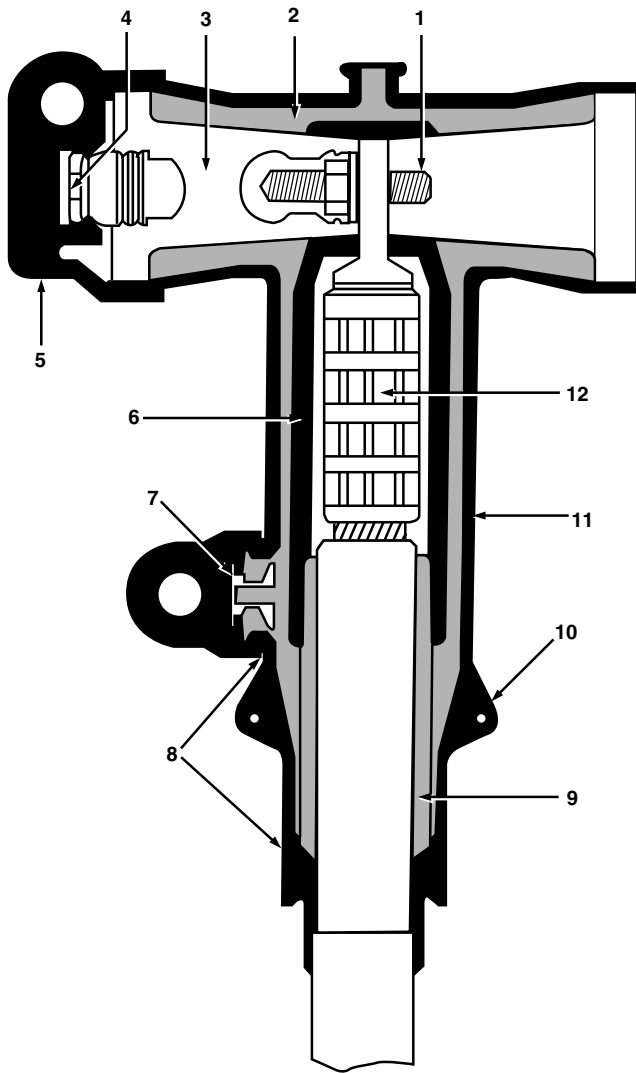
Figure 1. 1250 A, 24 kV Class DT612 deadbreak tee connector.
