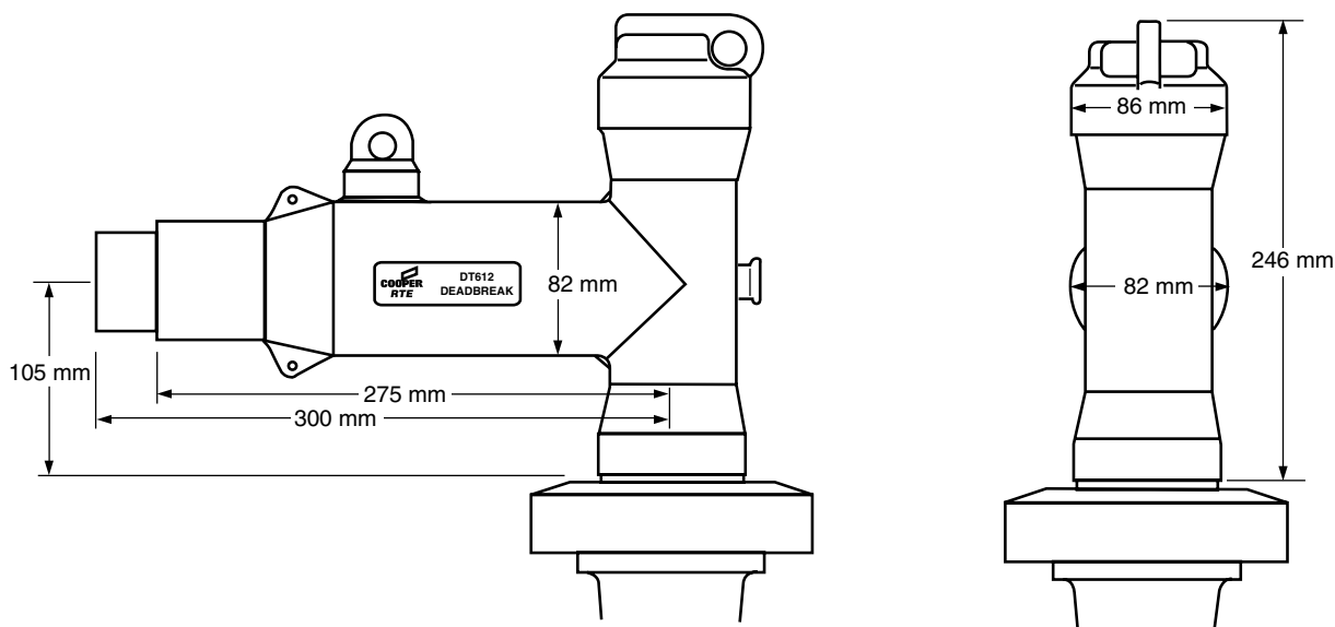
Figure 2. DT612 deadbreak tee connector.
