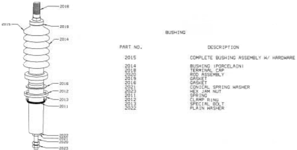
Figure 6-1. High-voltage bushing.
