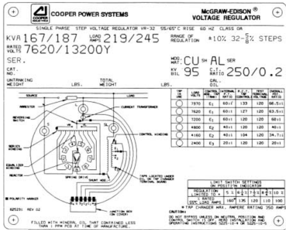
Figure 2-6. Nameplate.
