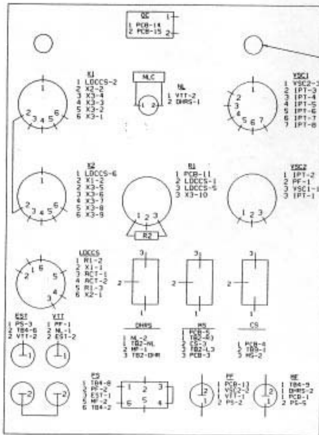
FRONT PANEL (VIEWED FROM REAR)
