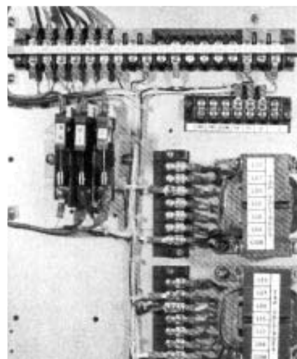
Figure 1-6. Knife switches and TB1 (with optional V6 knife switch and RCT2).
