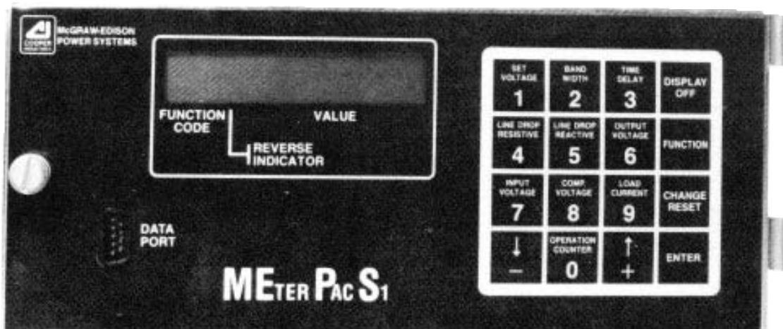
Figure 5-5. Meter Pac.
