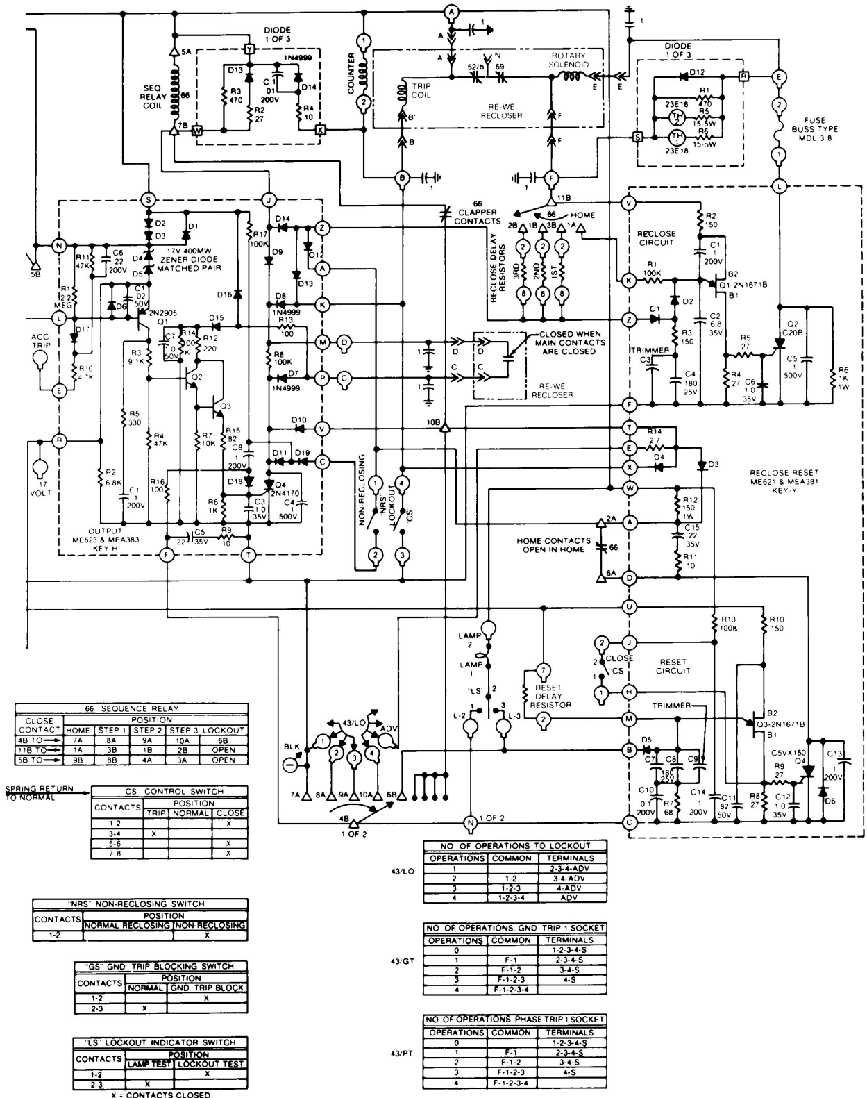
Figure 38b. Schematic diagram of Form 3 and RE/WE recloser (page 2 of 2).
