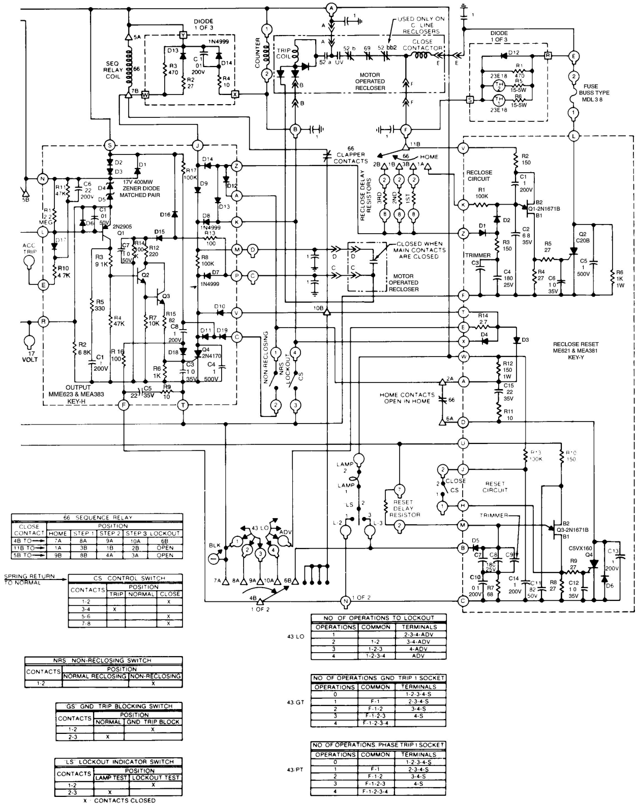
Figure 39b. Schematic diagram of Form 3 and motor operated recloser (page 2 of 2).
