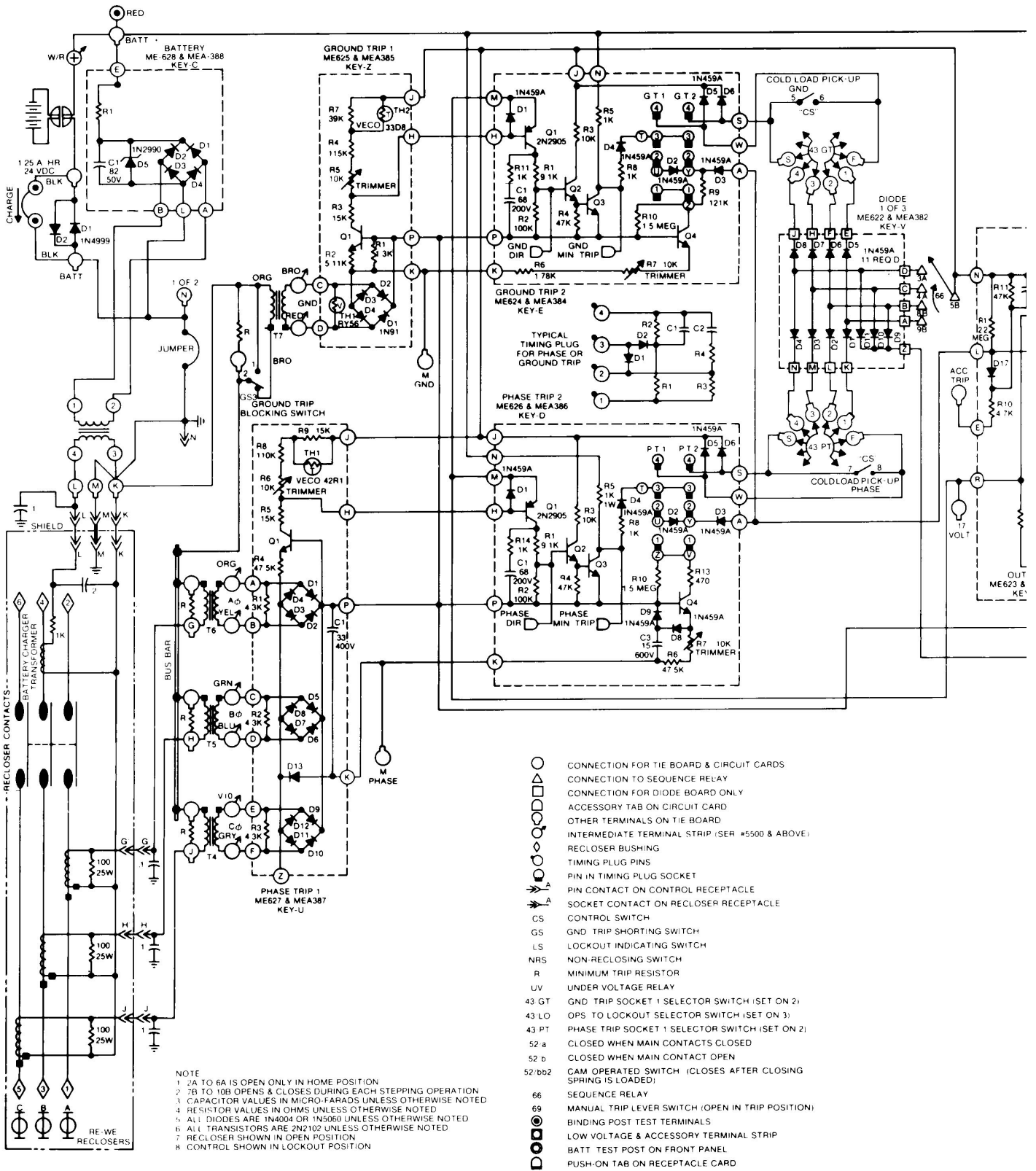
Figure 38a. Schematic diagram of Form 3 and RE/WE recloser (page 1 of 2).
