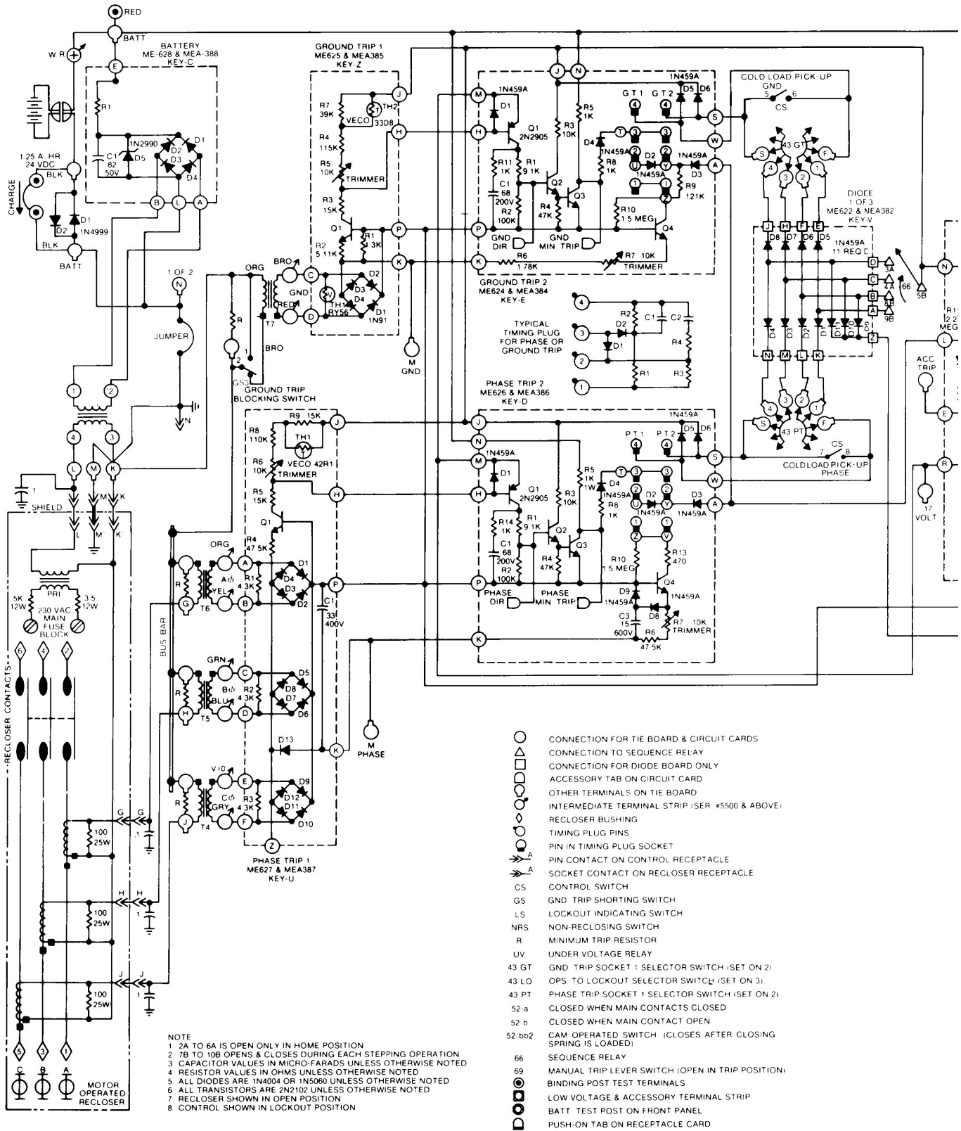
Figure 39a. Schematic diagram of Form 3 and motor operated recloser (page 1 of 2).
