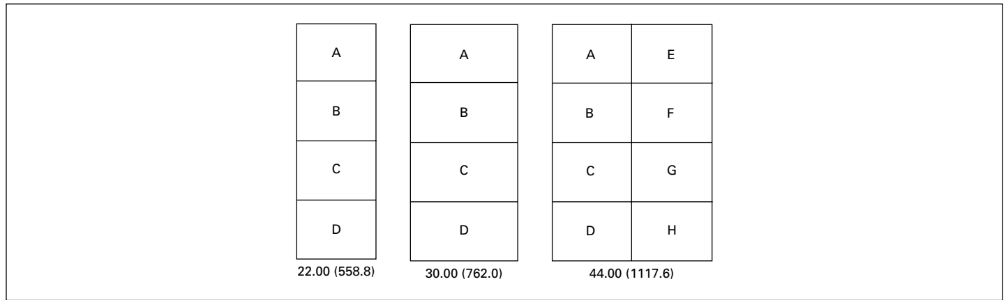
Figure 20.2-2. Breaker Structures—Dimensions in Inches (mm)
