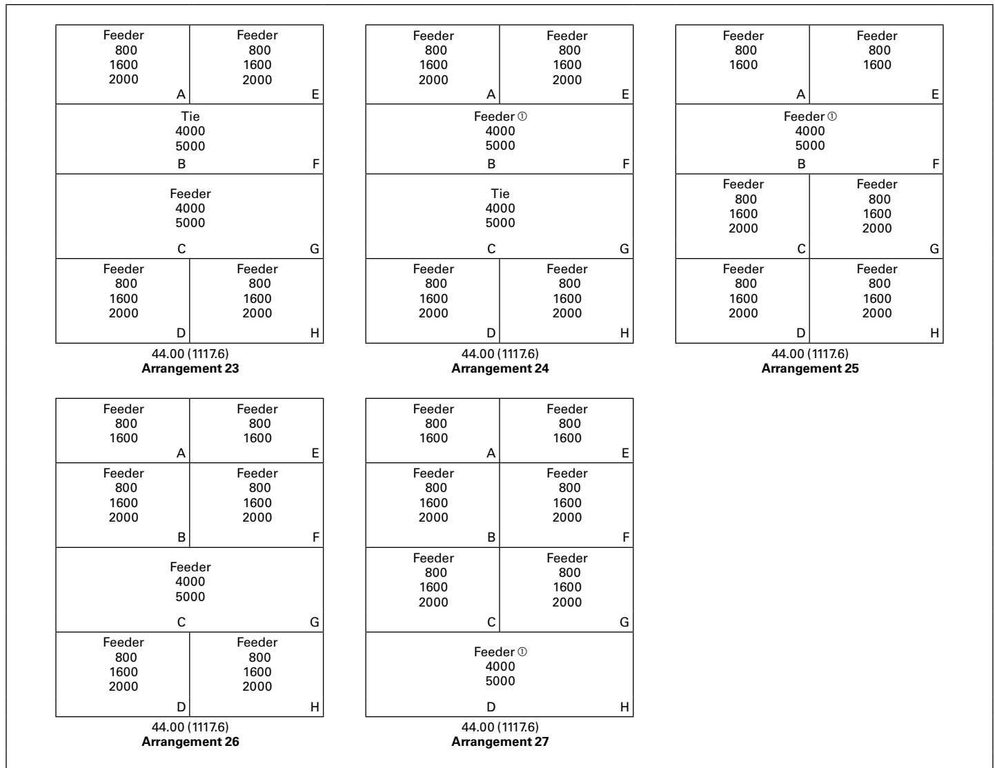
Figure 20.2-5. Typical Structure and Breaker Arrangements (Continued)—Magnum DS Ties and Feeders, 4000 A and 5000 A ②
