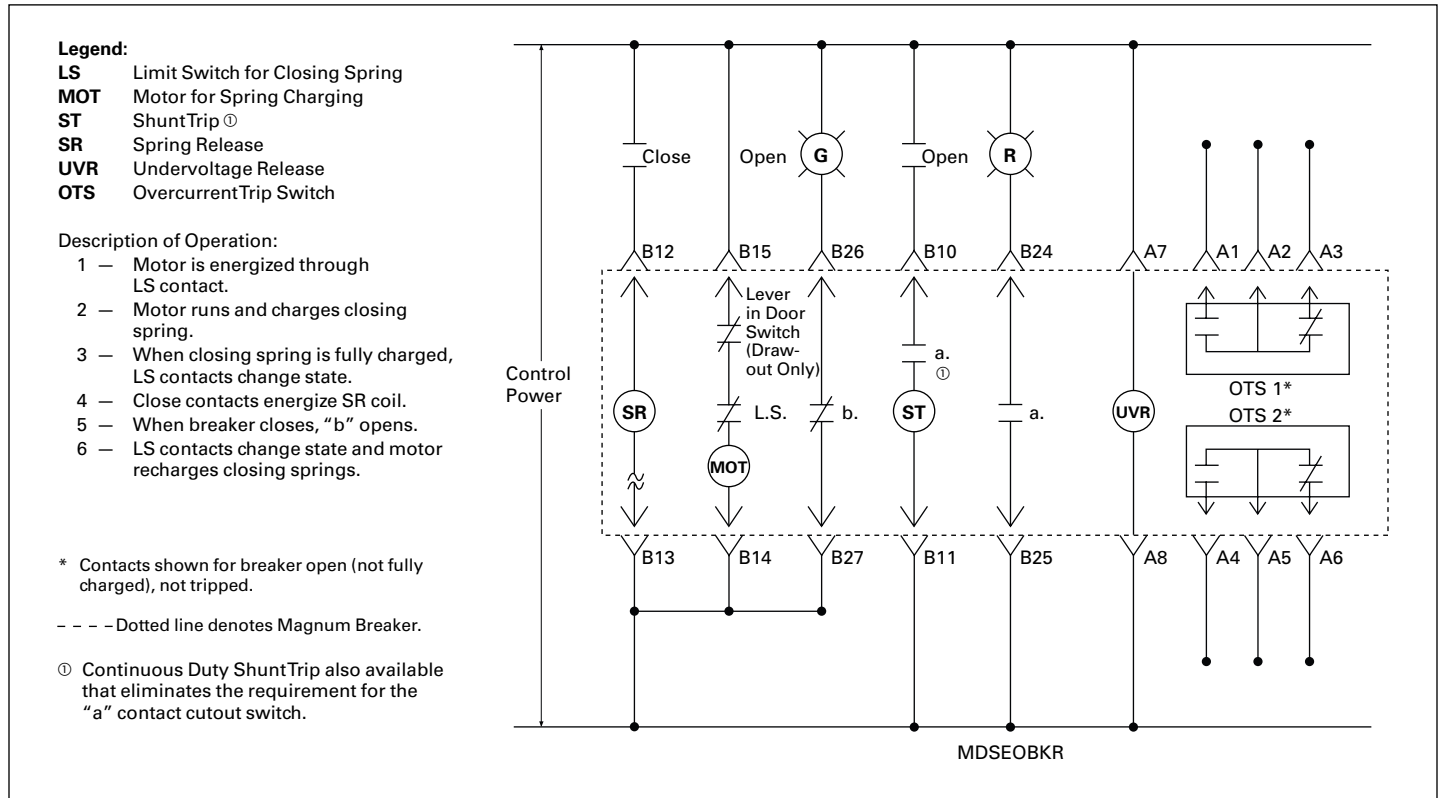
Figure 20.2-12. Typical Magnum Breaker Control Circuit Diagram
