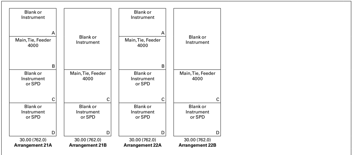
Figure 20.2-4. Typical Structure and Breaker Arrangements—4000 A, MDN Mains, Ties, Feeders and Miscellaneous—Dimensions in Inches (mm) Note: Minimum structure depth is 72 inches.
