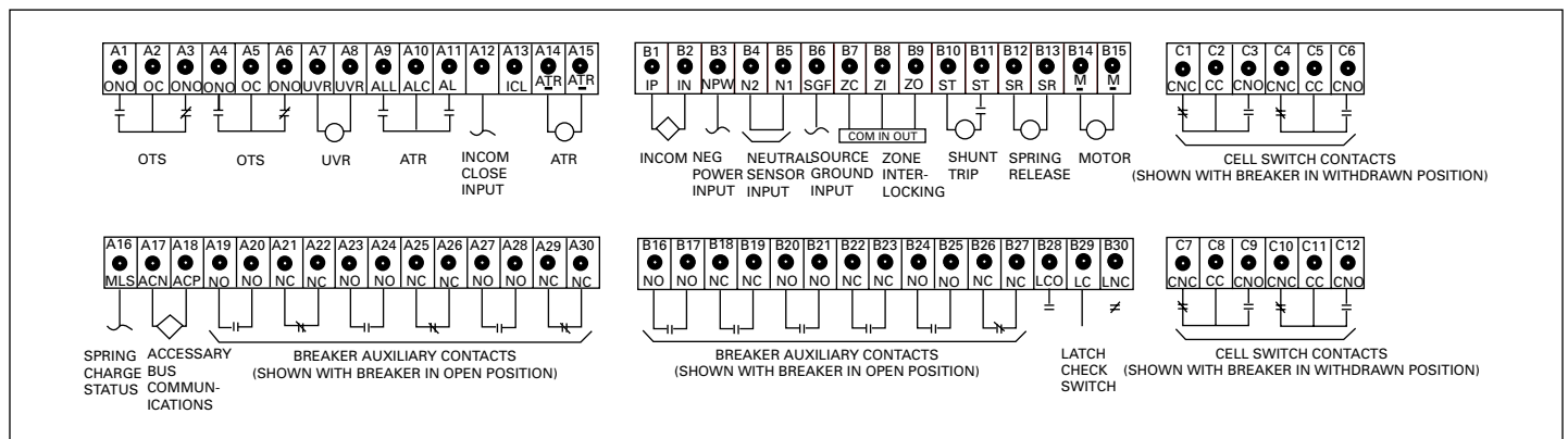
Figure 20.2-13. Typical Magnum Secondary Terminal Block Connection Diagram
