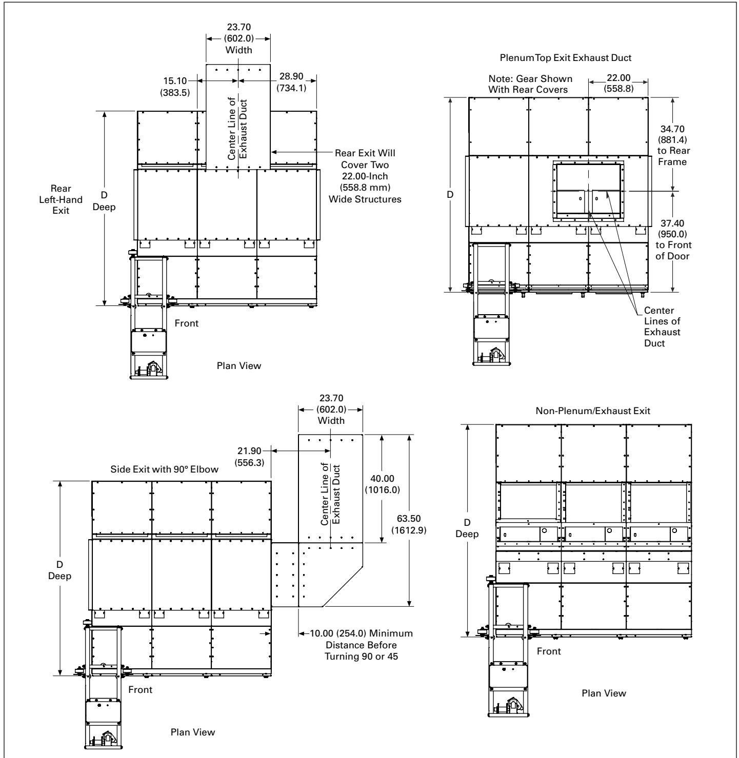
Figure 20.2-11. Arc-Resistant Switchgear Exhaust Configurations (Continued)
