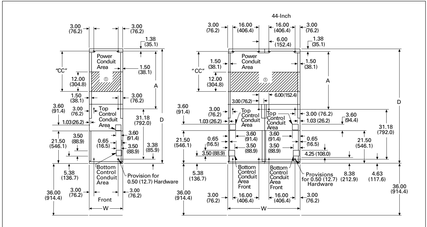
Figure 20.2-6. Floor Plans and Available Conduit Space—18.00, 22.00, 30.00, 44.00-Inch (457.2, 558.8, 762.0, 1117.6 mm) Wide Rear-Access Structures—Dimensions in Inches (mm)
