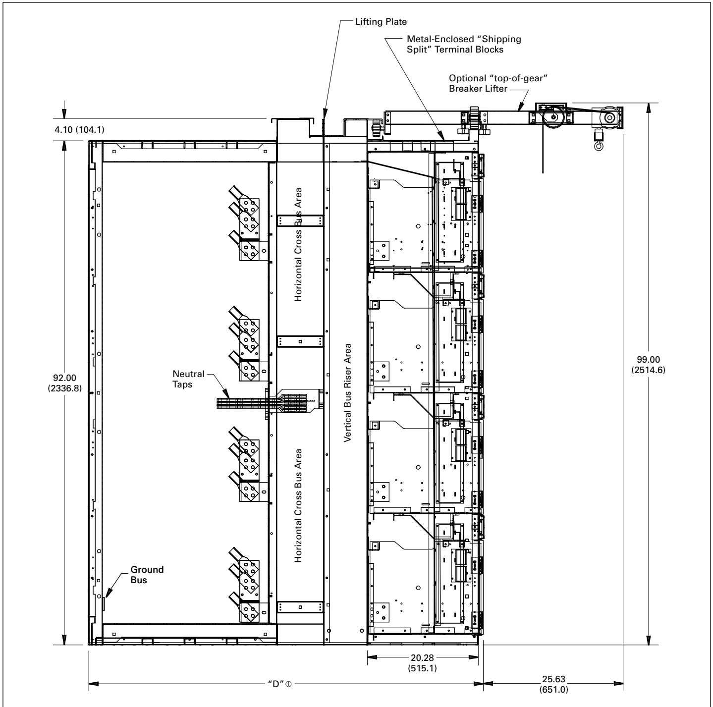
Figure 20.2-7. Section View of a Typical Structure with Magnum DS Breakers
