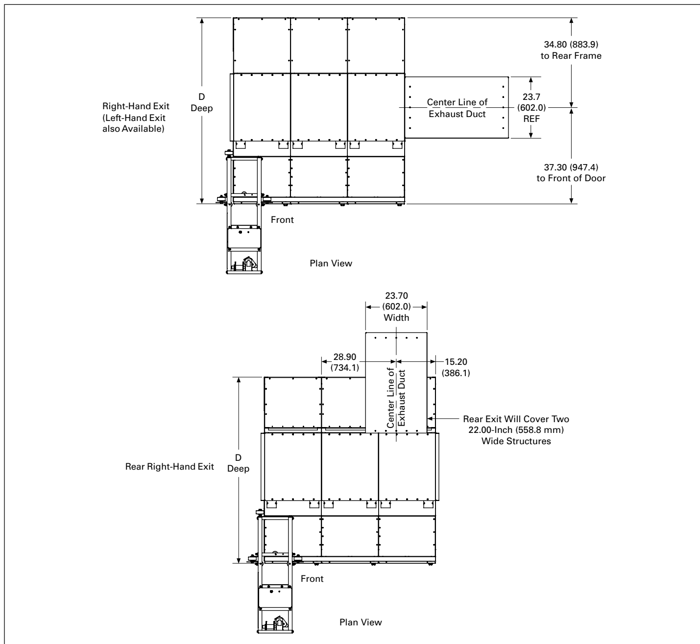
Figure 20.2-11. Arc-Resistant Switchgear Exhaust Configurations—Dimensions in Inches (mm)
