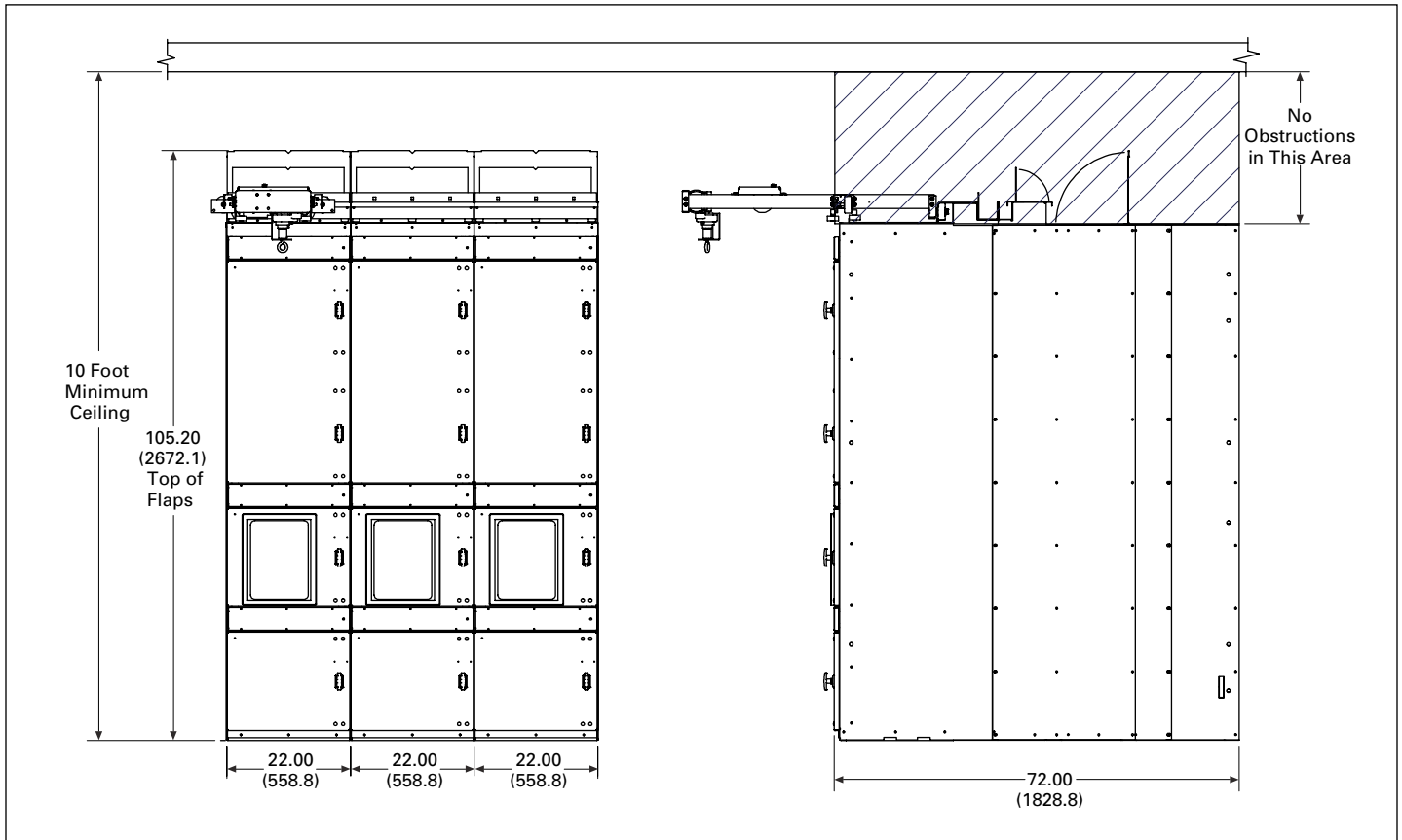
Figure 20.2-9. Non-Plenum Top Exit Configuration—Dimensions in Inches (mm)
