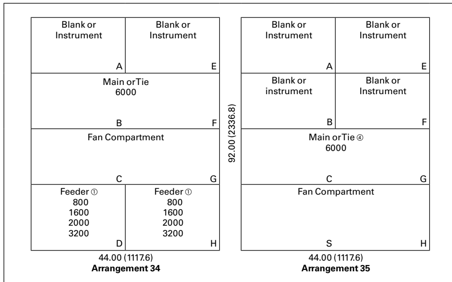
Figure 20.2-5. Typical Structure and Breaker Arrangements (Continued)— Magnum DS Mains and Ties, 6000 A ③
