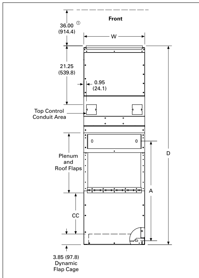
Figure 20.2-8. Arc-Resistant Structure Floor Plans and Available Conduit Space—Dimensions in Inches (mm)
