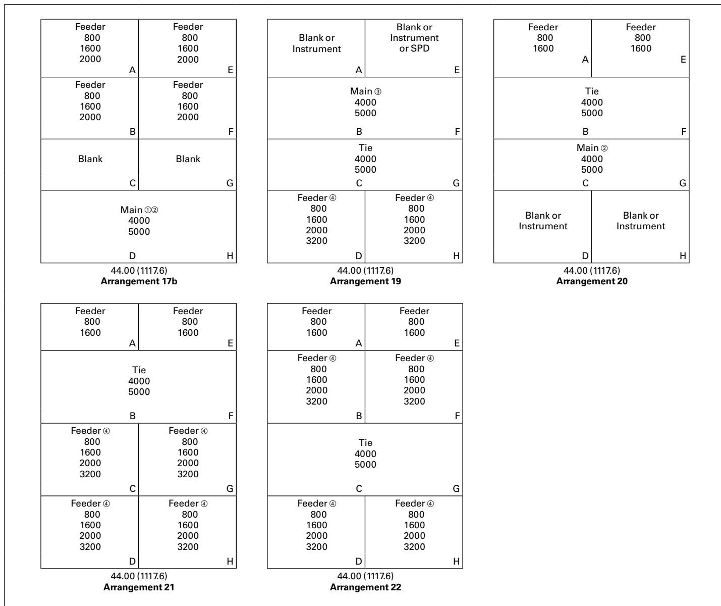
Figure 20.2-5. Typical Structure and Breaker Arrangements (Continued)—Magnum DS Mains and Ties, 4000 A and 5000 A ⑤
