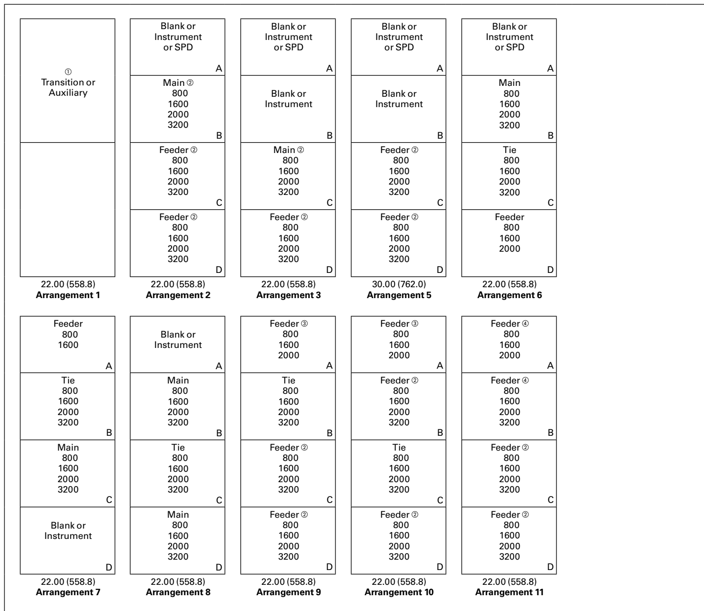
Figure 20.2-5. Typical Structure and Breaker Arrangements—Magnum DS Mains, Ties, Feeders and Miscellaneous, 3200 A and Below ⑤
