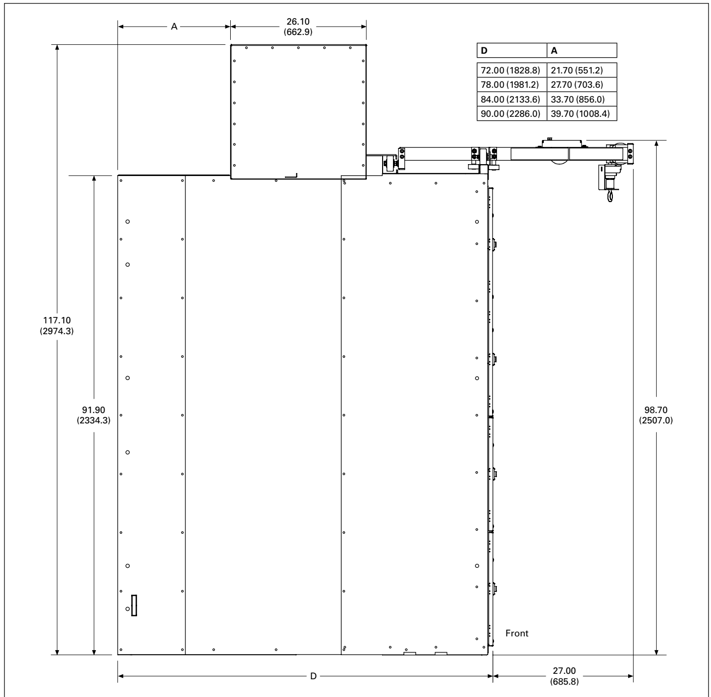
Figure 20.2-10. Arc-Resistant Switchgear Side View Showing the Arc Plenum—Dimensions in Inches (mm)
