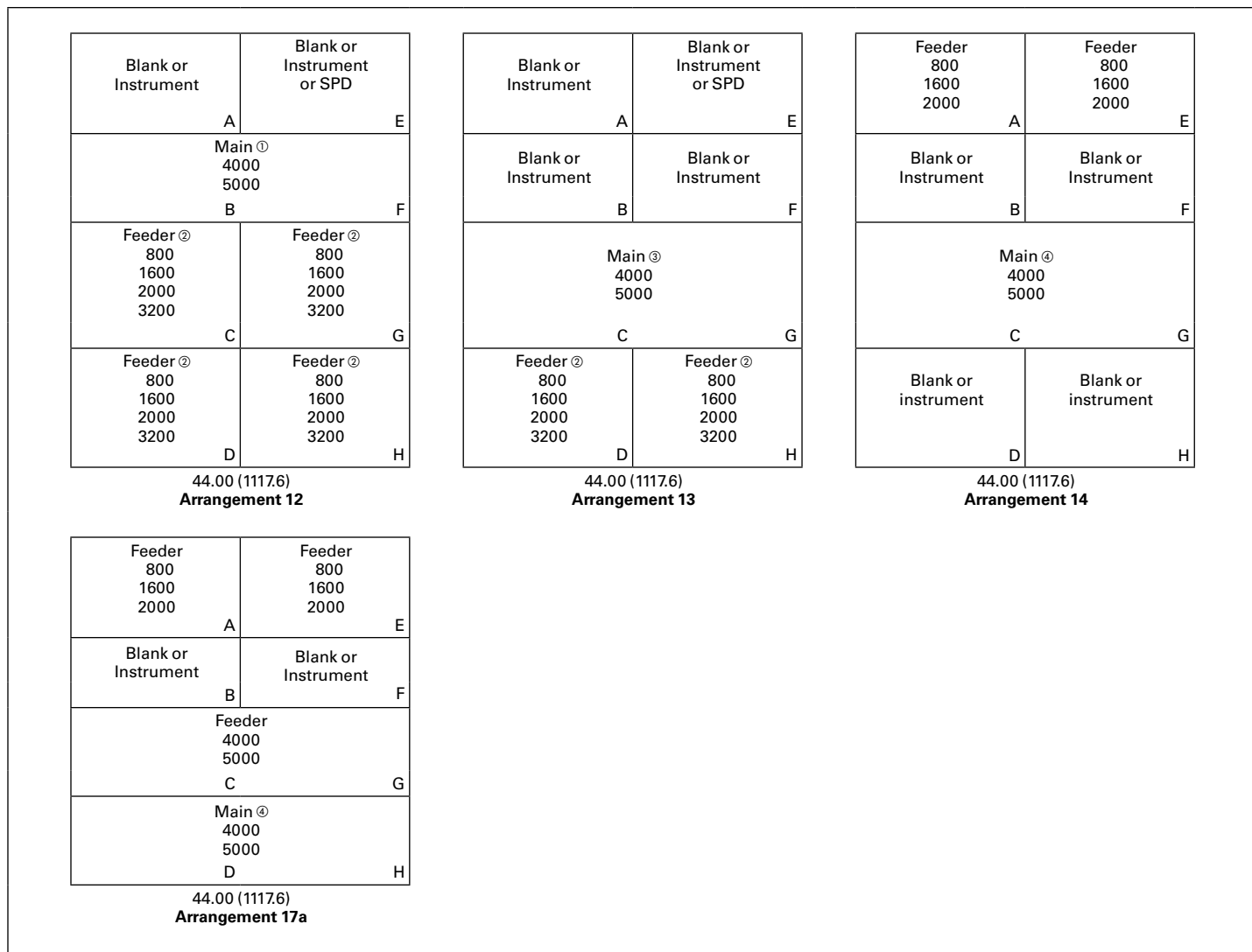
Figure 20.2-5. Typical Structure and Breaker Arrangements (Continued)—Magnum DS Mains, 4000 A and 5000 A
