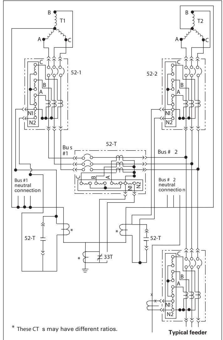
Figure 23. Four-wire double-ended unit substation
