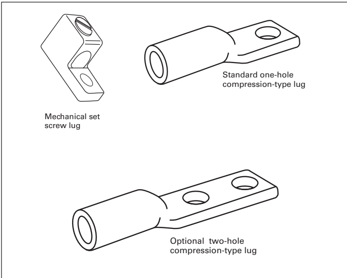
Figure 13. Screw and compression lugs
