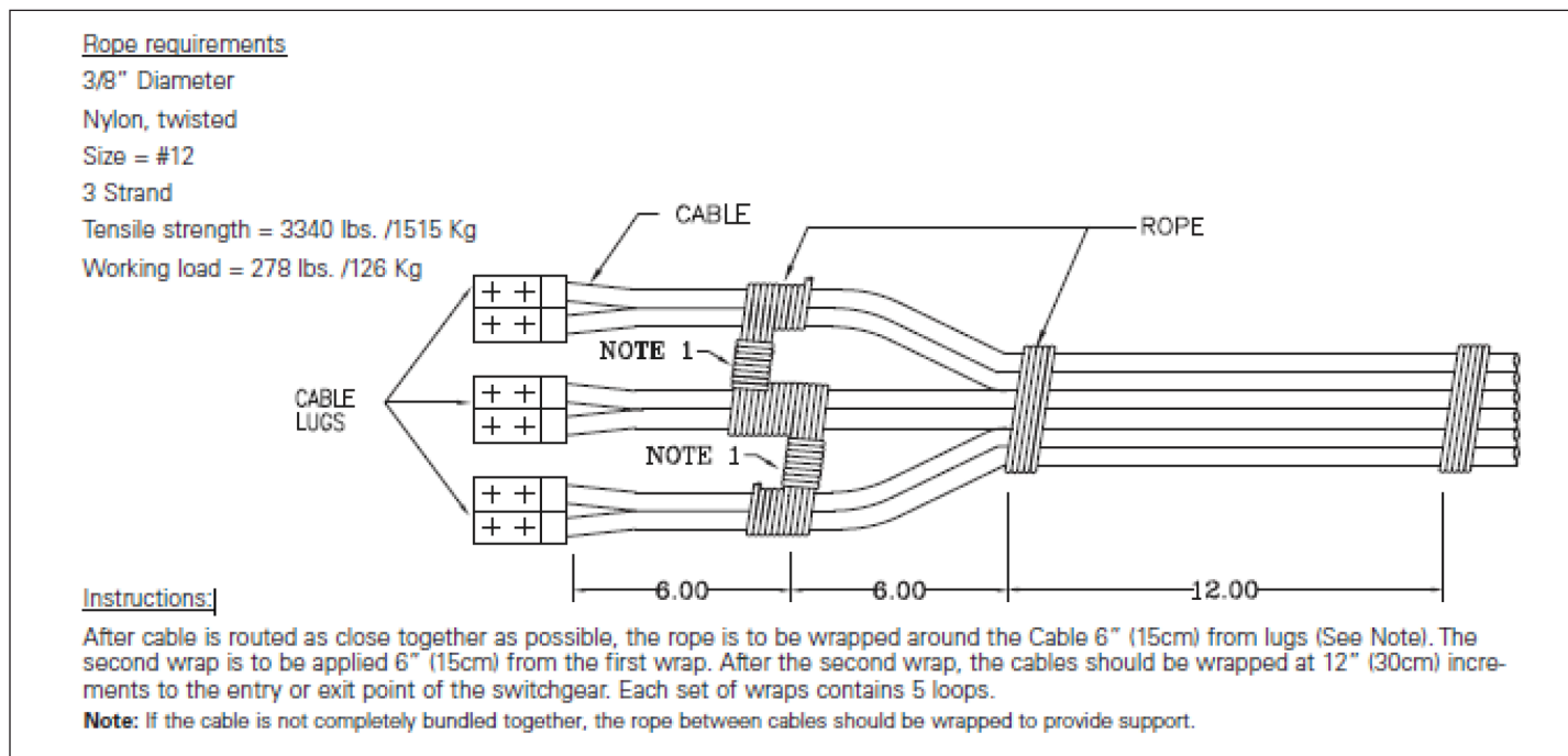
Figure 14. Cable lashing instructions
