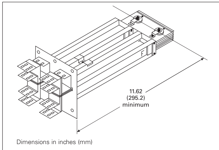
Figure 16. Standard flange
