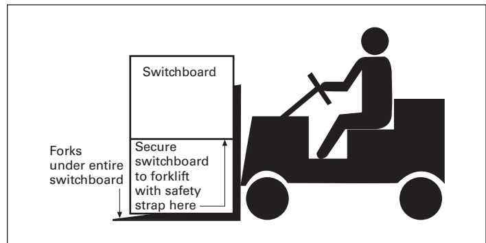
Figure 4. Forklift
