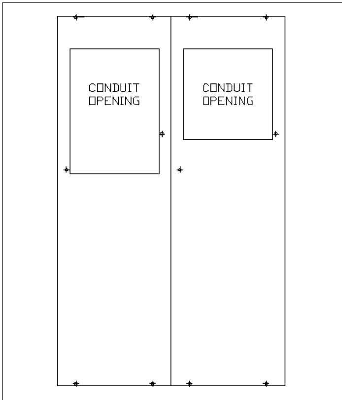
Figure 5. Conduit space drawing—floor plan
