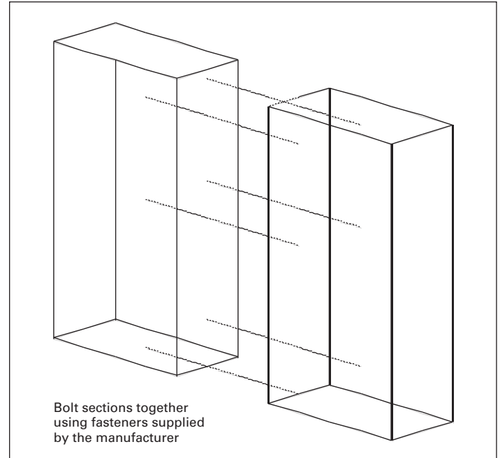
Figure 11. Joining switchboard sections
