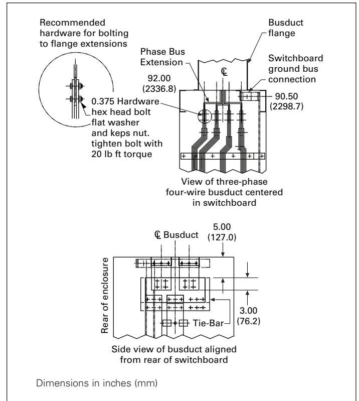
Figure 17. Busway/busduct
