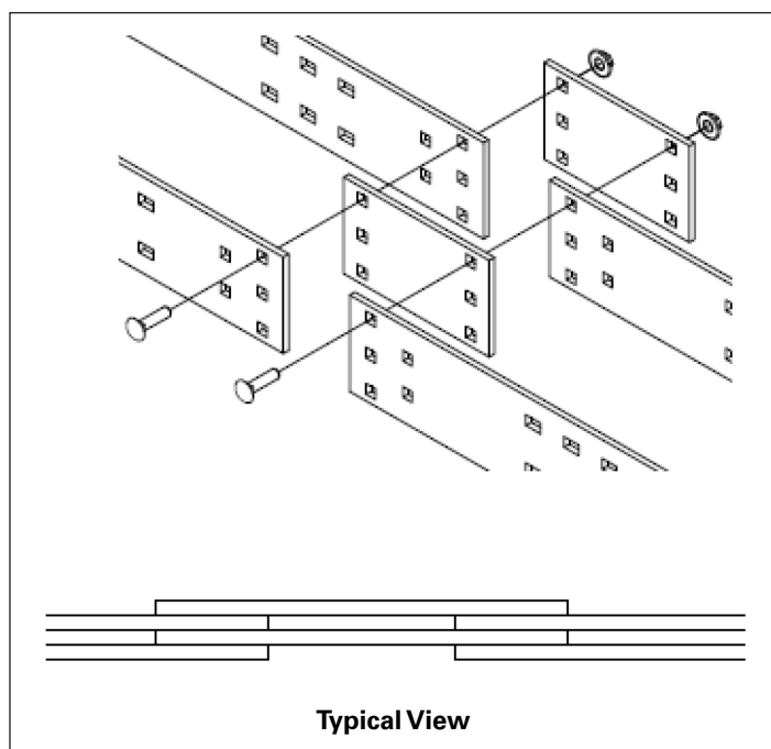
Figure 12. Splice plates
