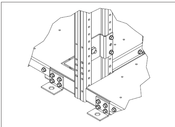
Figure 10. Switchboard section connection
