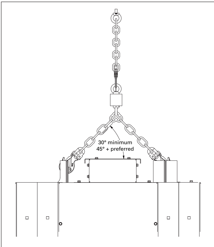
Figure 3. Side view
