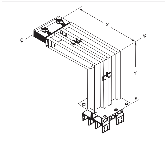
Figure 15. Downward elbow right flange
