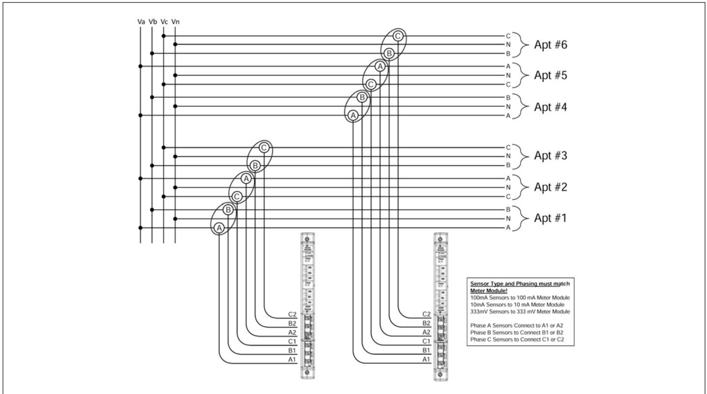
Figure 10. Network 120/208 Three-Wire Apartment Service Current Sensor Connections
