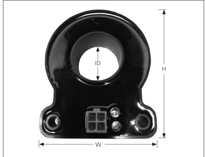
Figure 5. Current Sensor Dimensions
