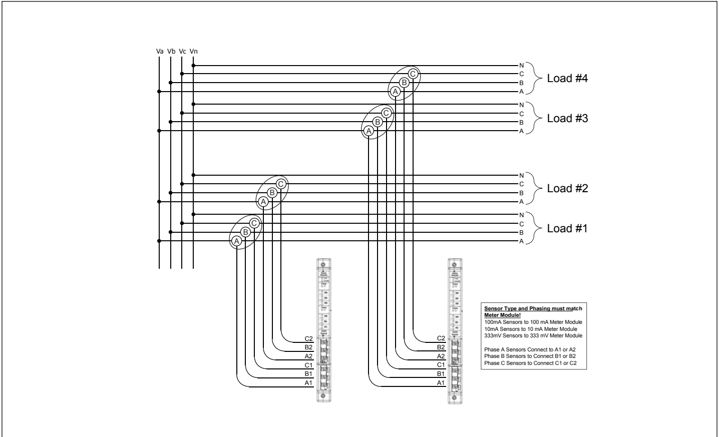
Figure 11. Typical Wiring – 3-Phase 4-Wire Wye.
