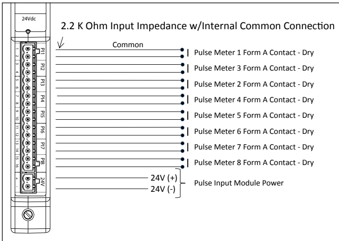
Figure 21. PXMP-PIM Wiring.
