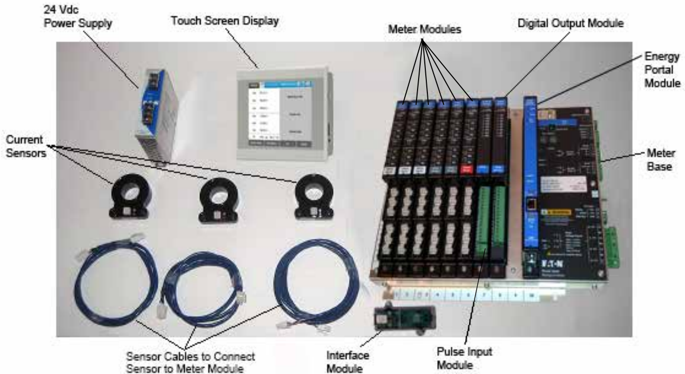
Figure 1. Components of the PXMP Meter System.
