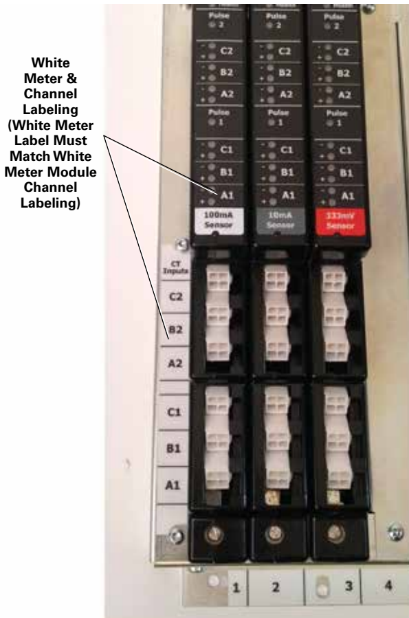
Figure 8. PXMP-MB Examples.
