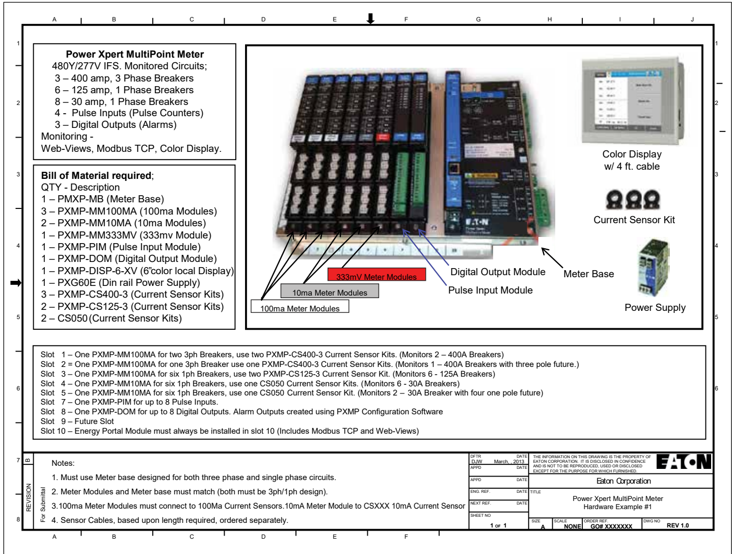
Figure 2. Example PXMP Meter Configuration.
