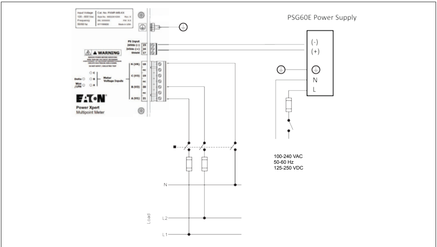
Figure 12. Typical Wiring – Single-Phase 3-Wire 120/240.
