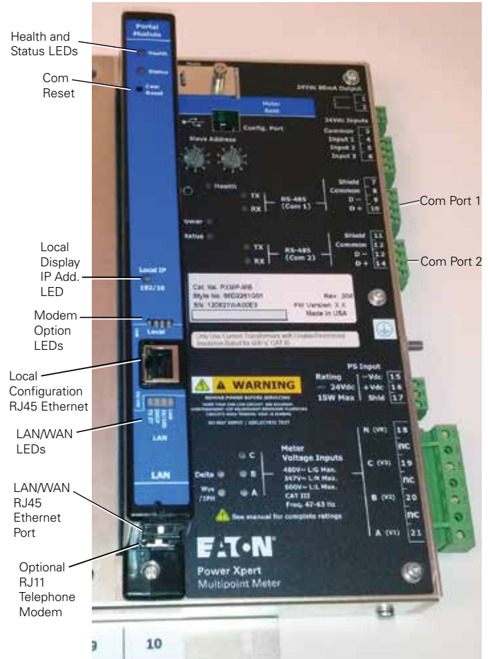
Figure 24. PXMP-EPM.
