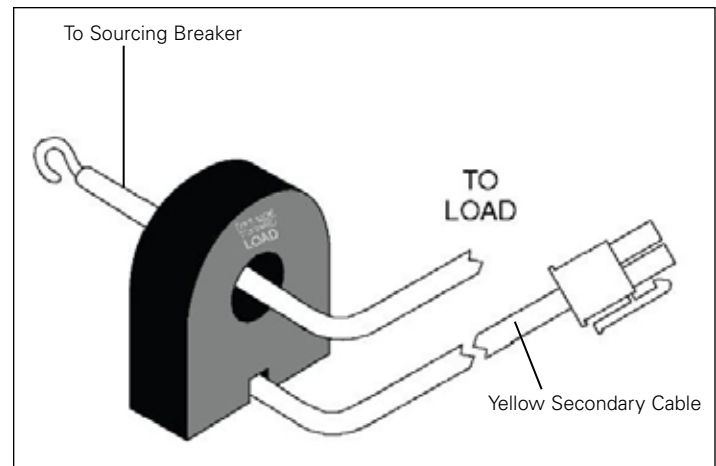
Figure 17. CS050/125/200/400 Current Sensors – Load Orientation.
