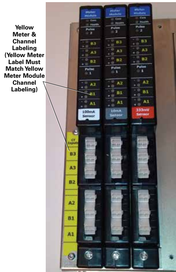
Figure 10. .PXMP-MB-AB Examples.
