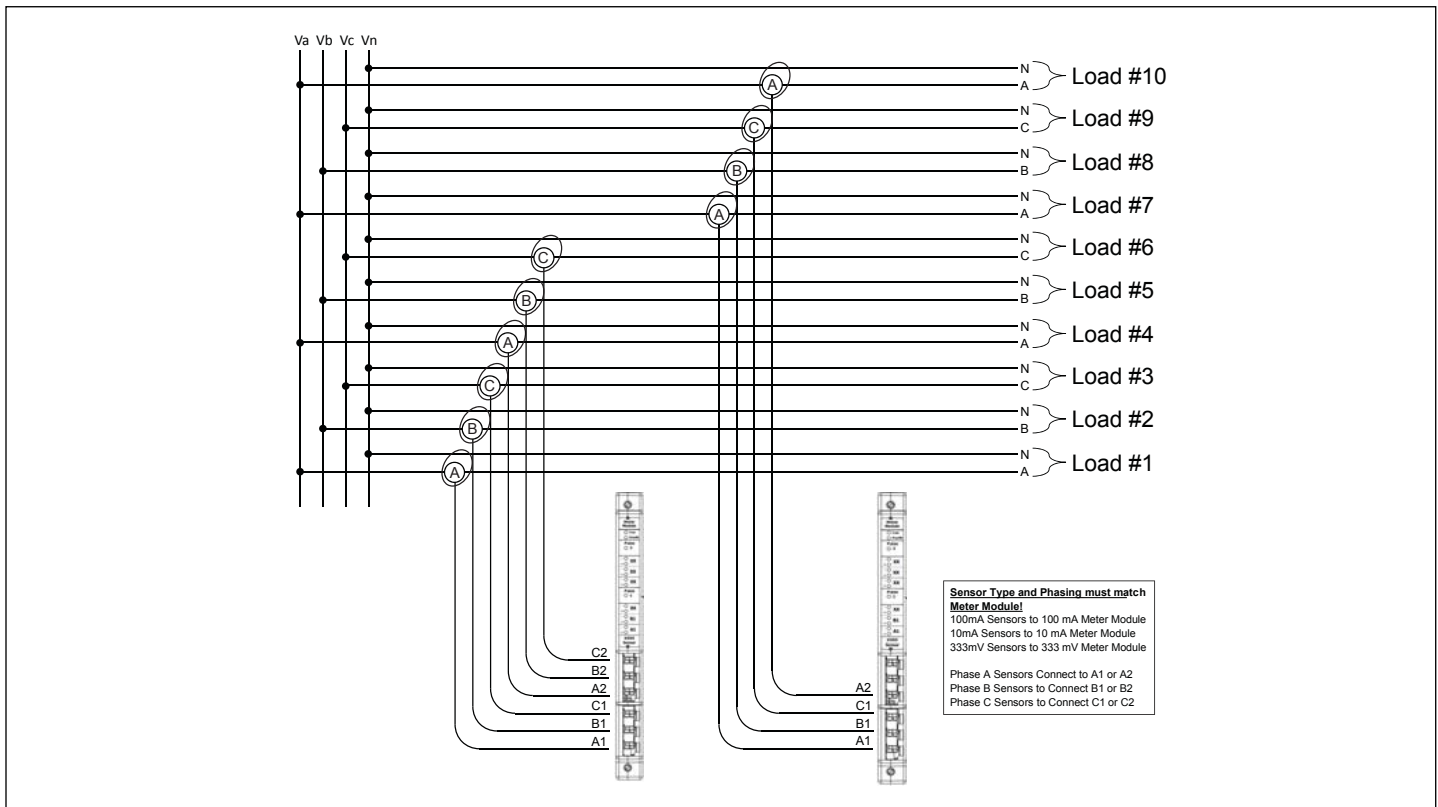
Figure 19. 3-Phase 4-Wire Service Using Ten Single-Phase, 1 Pole Current Sensors.
