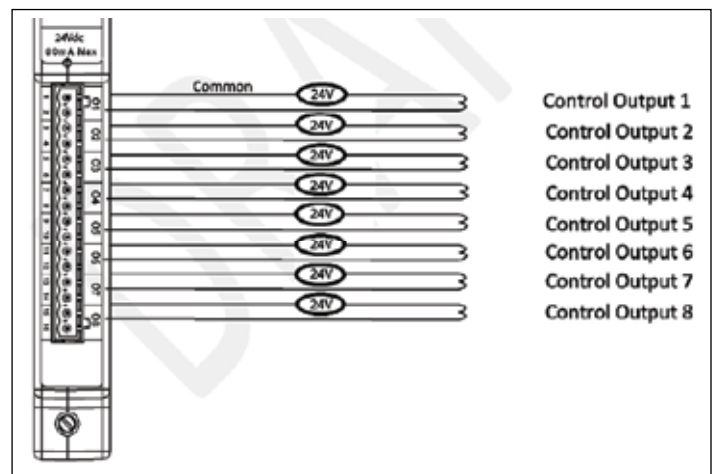
Figure 23. PXMP-DOM Wiring.
