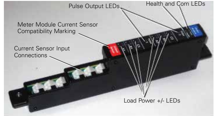
Figure 9. Typical PXMP-MM.
