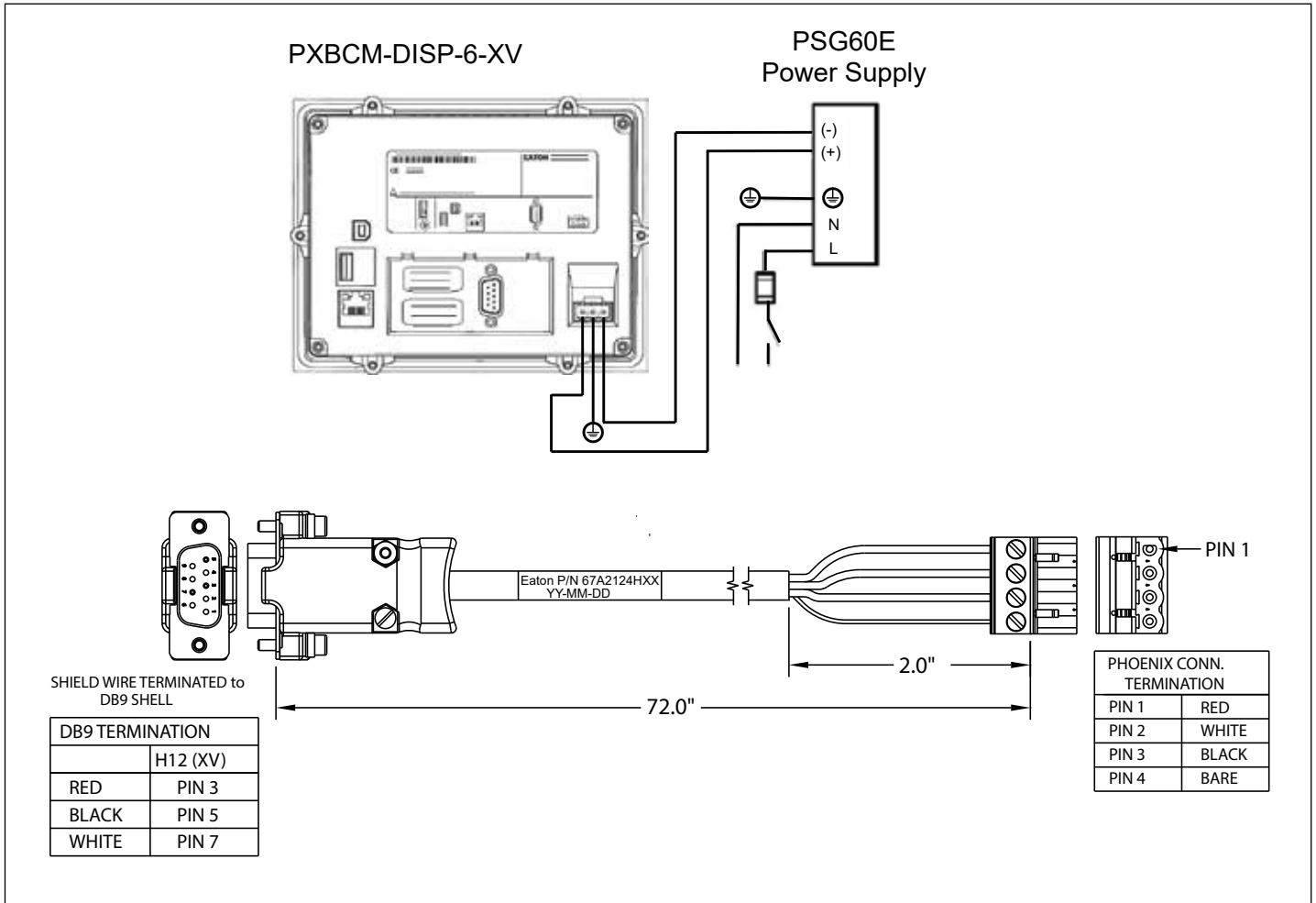
Figure 25. PXMP Touch Screen Display and Wiring Information.
