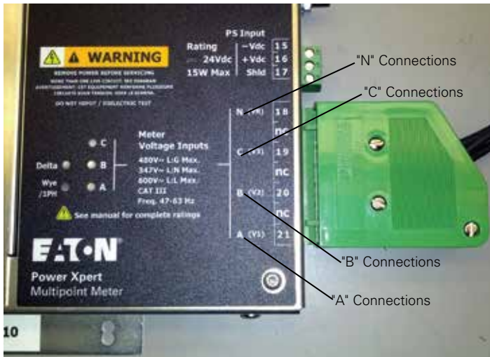
Figure 6. A, B, C, and N Connections on the PXMP-MB Assembly Meter Voltage Input.
