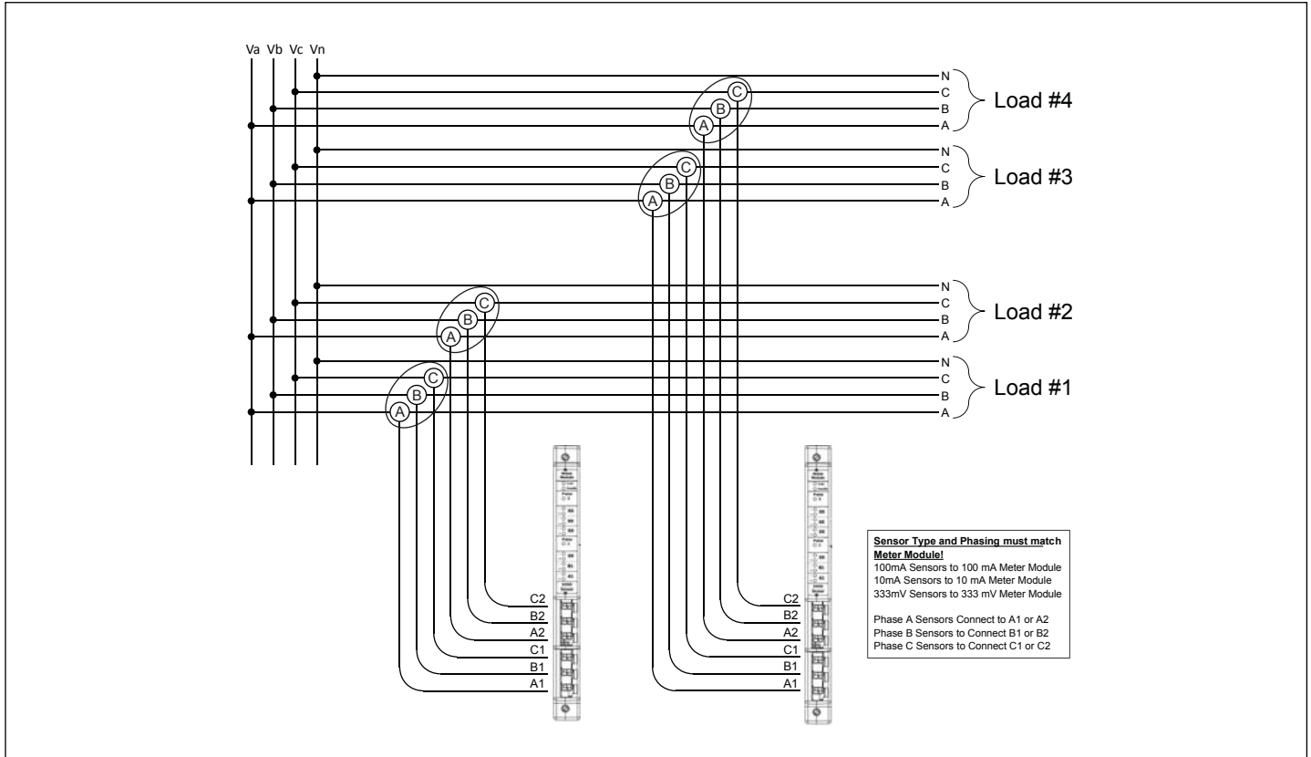
Figure 18. 3-Phase 4-Wire Service Using Two 3-Phase Current Sensors.
