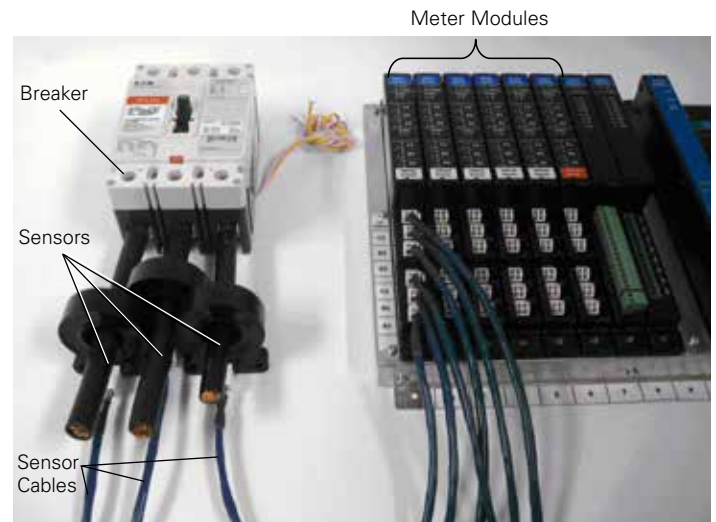
Figure 16. Typical Wiring Arrangement of Sensor Connected to Meter Module.
